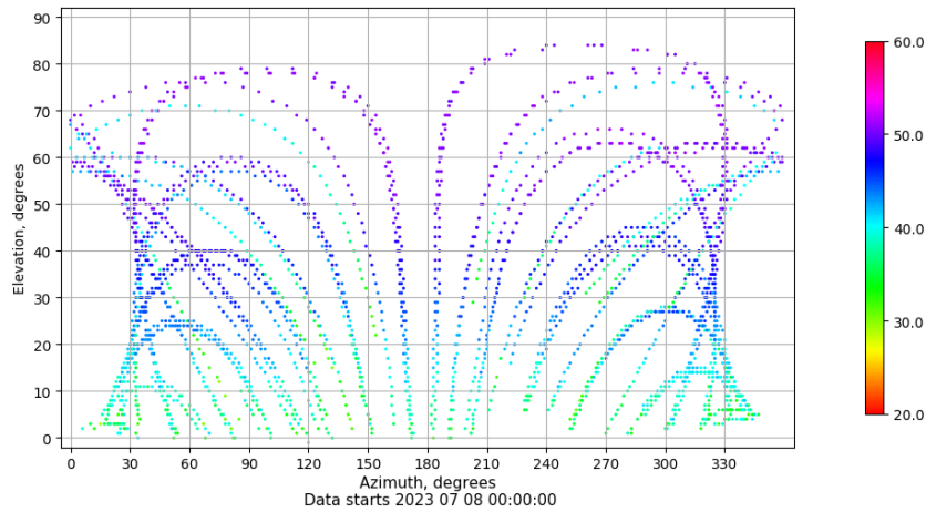
Azimuth-elevation plot for station BCL1. Signal to Noise S1C Data file BCL100ESP_R_2023189.xtr
