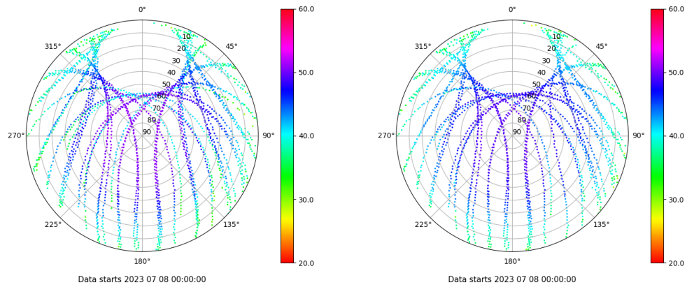
Skyplot for station BCL1. Signal to Noise S1C Data file BCL100ESP_R_2023189.xtr Skyplot for station BCL1. Signal to Noise S2P Data file BCL100ESP_R_2023189.xtr
