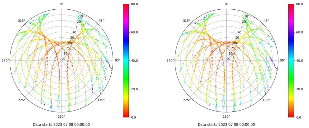
Skyplot for station BCL1. Parameter M1C Data file BCL100ESP_R_2023189.xtr Skyplot for station BCL1. Parameter M2P Data file BCL100ESP_R_2023189.xtr
