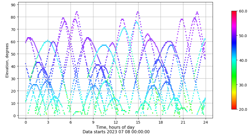
Time-elevation plot for station BCL1. Signal to Noise S1C Data file BCL100ESP_R_2023189.xtr
