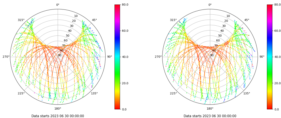
Skyplot for station BCL1. Parameter M1C Data file BCL100ESP_R_2023181.xtr Skyplot for station BCL1. Parameter M2W Data file BCL100ESP_R_2023181.xtr
