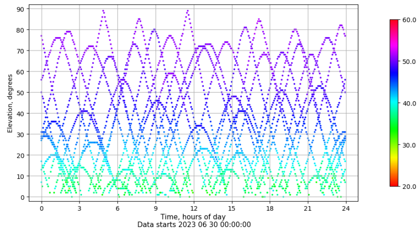
Time-elevation plot for station BCL1. Signal to Noise S1C Data file BCL100ESP_R_2023181.xtr
