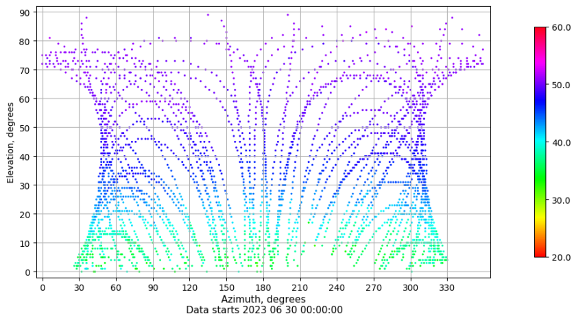
Azimuth-elevation plot for station BCL1. Signal to Noise S1C Data file BCL100ESP_R_2023181.xtr
