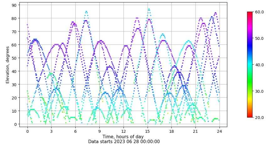
Time-elevation plot for station BCL1. Signal to Noise S1C Data file BCL100ESP_R_2023179.xtr
