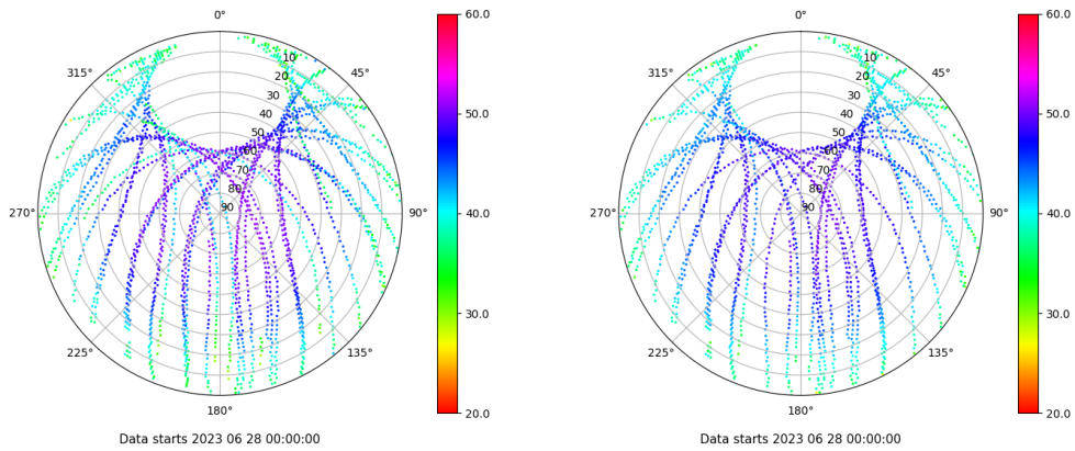
Skyplot for station BCL1. Signal to Noise S1C Data file BCL100ESP_R_2023179.xtr Skyplot for station BCL1. Signal to Noise S2P Data file BCL100ESP_R_2023179.xtr
