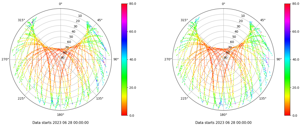
Skyplot for station BCL1. Parameter M1C Data file BCL100ESP_R_2023179.xtr Skyplot for station BCL1. Parameter M2W Data file BCL100ESP_R_2023179.xtr
