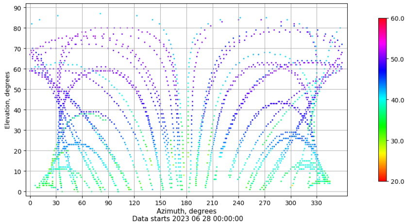
Azimuth-elevation plot for station BCL1. Signal to Noise S1C Data file BCL100ESP_R_2023179.xtr
