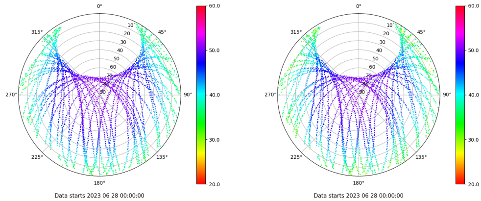
Skyplot for station BCL1. Signal to Noise S1C Data file BCL100ESP_R_2023179.xtr Skyplot for station BCL1. Signal to Noise S2W Data file BCL100ESP_R_2023179.xtr
