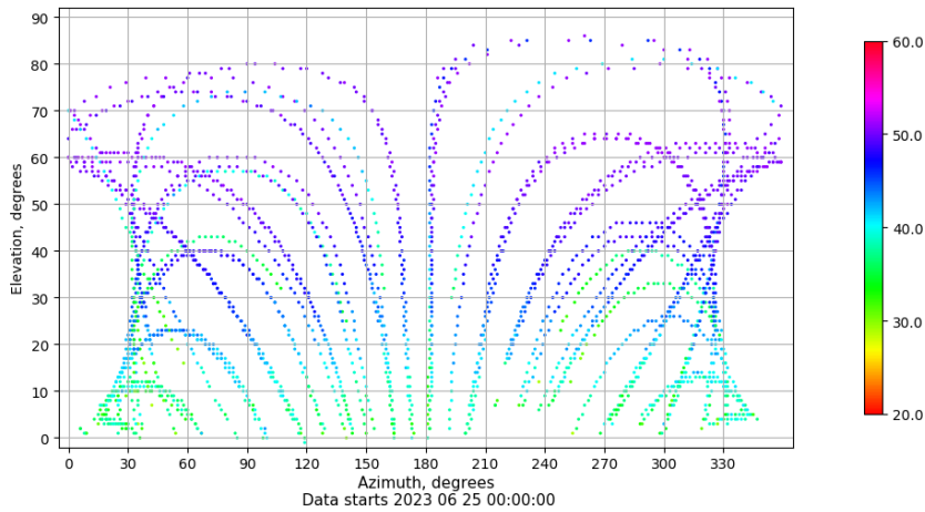
Azimuth-elevation plot for station BCL1. Signal to Noise S1C Data file BCL100ESP_R_2023176.xtr
