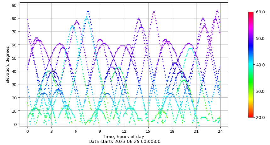
Time-elevation plot for station BCL1. Signal to Noise S1C Data file BCL100ESP_R_2023176.xtr
