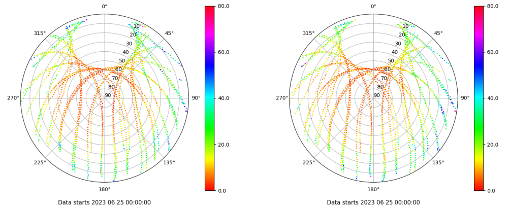
Skyplot for station BCL1. Parameter M1C Data file BCL100ESP_R_2023176.xtr Skyplot for station BCL1. Parameter M2P Data file BCL100ESP_R_2023176.xtr
