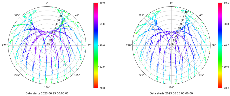
Skyplot for station BCL1. Signal to Noise S1C Data file BCL100ESP_R_2023176.xtr Skyplot for station BCL1. Signal to Noise S2P Data file BCL100ESP_R_2023176.xtr
