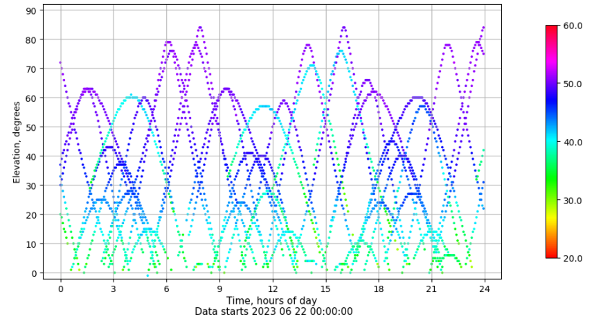
Time-elevation plot for station BCL1. Signal to Noise S1C Data file BCL100ESP_R_2023173.xtr
