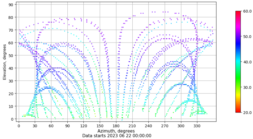
Azimuth-elevation plot for station BCL1. Signal to Noise S1C Data file BCL100ESP_R_2023173.xtr
