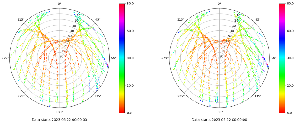
Skyplot for station BCL1. Parameter M1C Data file BCL100ESP_R_2023173.xtr Skyplot for station BCL1. Parameter M2P Data file BCL100ESP_R_2023173.xtr
