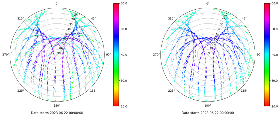
Skyplot for station BCL1. Signal to Noise S1C Data file BCL100ESP_R_2023173.xtr Skyplot for station BCL1. Signal to Noise S2P Data file BCL100ESP_R_2023173.xtr
