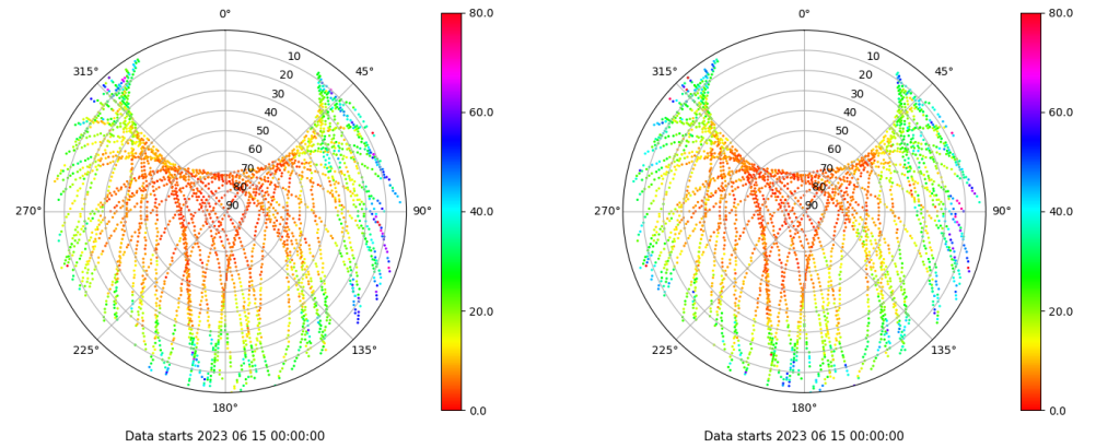
Skyplot for station BCL1. Parameter M1C Data file BCL100ESP_R_2023166.xtr Skyplot for station BCL1. Parameter M2W Data file BCL100ESP_R_2023166.xtr
