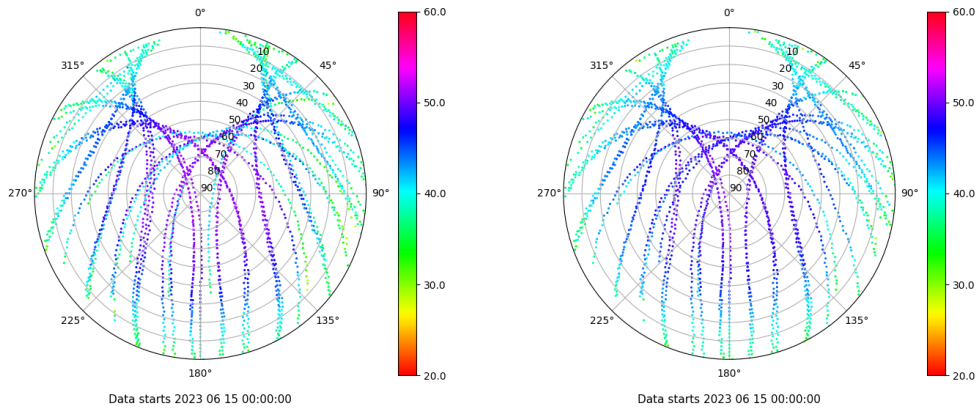
Skyplot for station BCL1. Signal to Noise S1C Data file BCL100ESP_R_2023166.xtr Skyplot for station BCL1. Signal to Noise S2P Data file BCL100ESP_R_2023166.xtr
