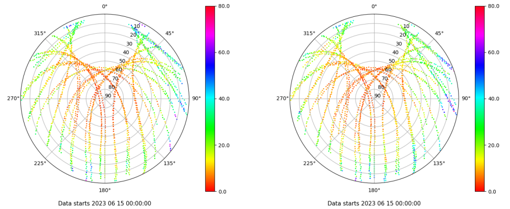
Skyplot for station BCL1. Parameter M1C Data file BCL100ESP_R_2023166.xtr Skyplot for station BCL1. Parameter M2P Data file BCL100ESP_R_2023166.xtr
