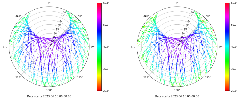
Skyplot for station BCL1. Signal to Noise S1C Data file BCL100ESP_R_2023166.xtr Skyplot for station BCL1. Signal to Noise S2W Data file BCL100ESP_R_2023166.xtr
