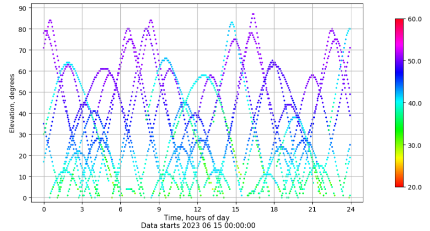
Time-elevation plot for station BCL1. Signal to Noise S1C Data file BCL100ESP_R_2023166.xtr
