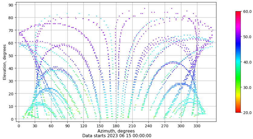
Azimuth-elevation plot for station BCL1. Signal to Noise S1C Data file BCL100ESP_R_2023166.xtr
