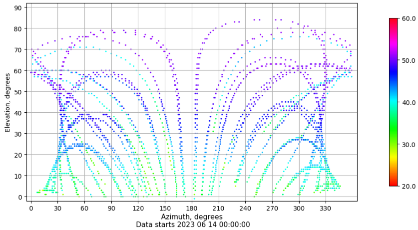
Azimuth-elevation plot for station BCL1. Signal to Noise S1C Data file BCL100ESP_R_2023165.xtr
