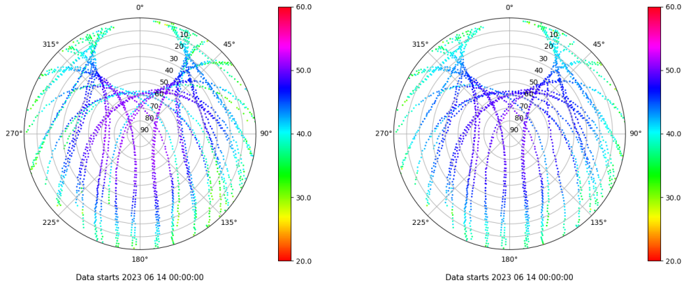
Skyplot for station BCL1. Signal to Noise S1C Data file BCL100ESP_R_2023165.xtr Skyplot for station BCL1. Signal to Noise S2P Data file BCL100ESP_R_2023165.xtr
