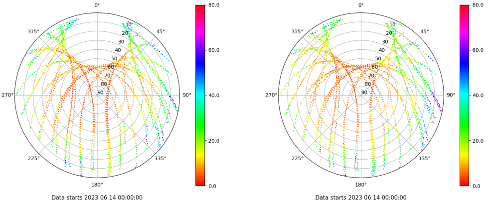
Skyplot for station BCL1. Parameter M1C Data file BCL100ESP_R_2023165.xtr Skyplot for station BCL1. Parameter M2P Data file BCL100ESP_R_2023165.xtr
