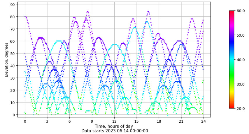
Time-elevation plot for station BCL1. Signal to Noise S1C Data file BCL100ESP_R_2023165.xtr
