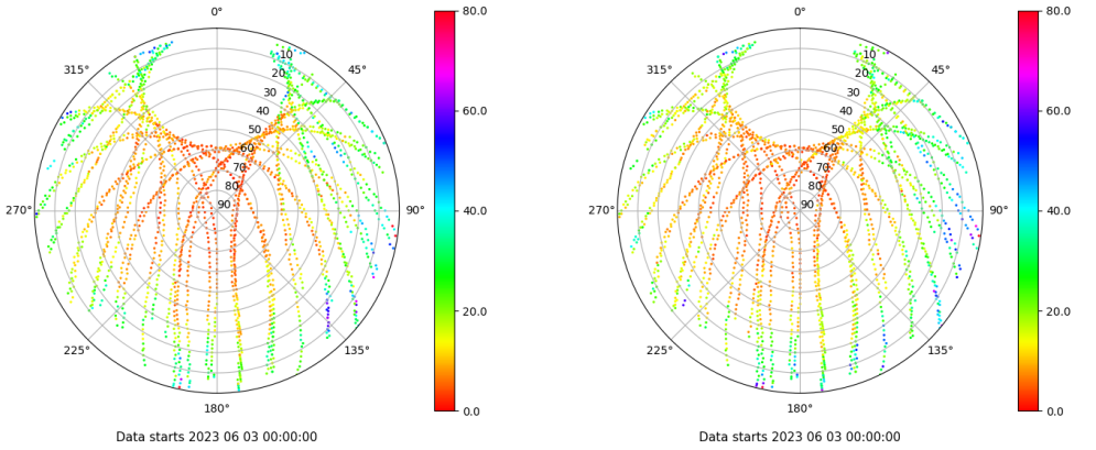
Skyplot for station BCL1. Parameter M1C Data file BCL100ESP_R_2023154.xtr Skyplot for station BCL1. Parameter M2P Data file BCL100ESP_R_2023154.xtr
