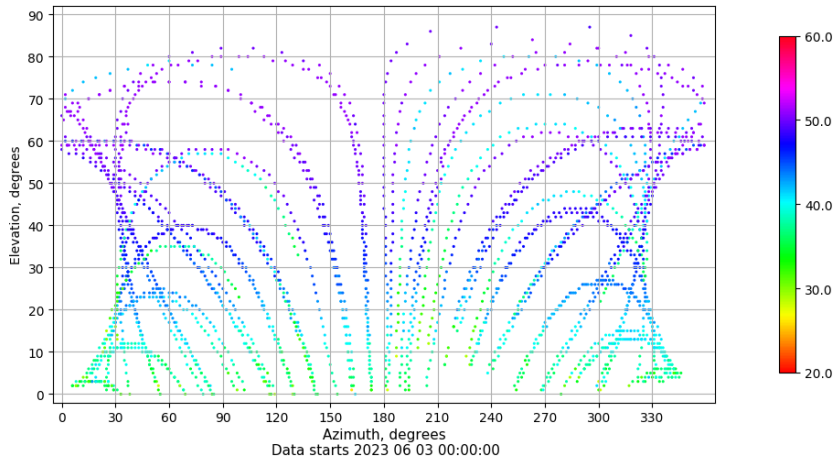
Azimuth-elevation plot for station BCL1. Signal to Noise S1C Data file BCL100ESP_R_2023154.xtr
