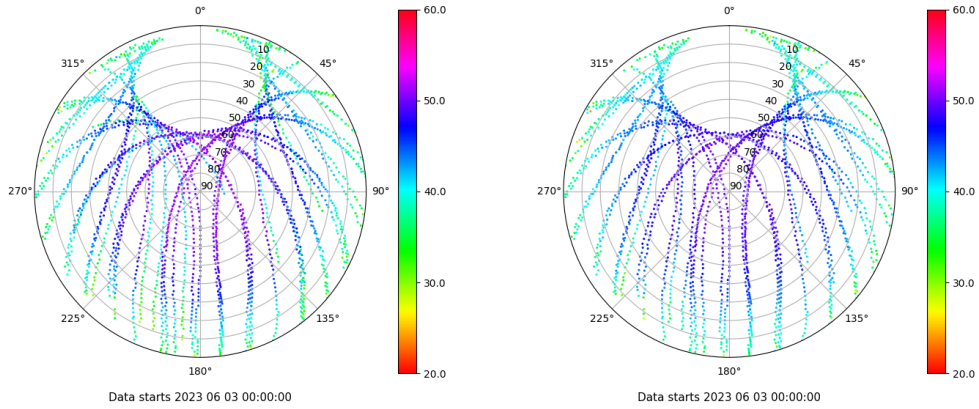
Skyplot for station BCL1. Signal to Noise S1C Data file BCL100ESP_R_2023154.xtr Skyplot for station BCL1. Signal to Noise S2P Data file BCL100ESP_R_2023154.xtr
