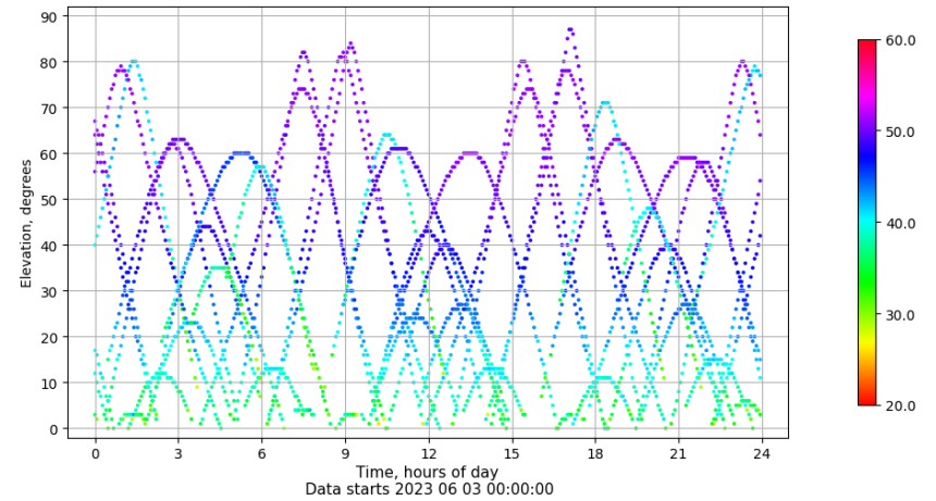
Time-elevation plot for station BCL1. Signal to Noise S1C Data file BCL100ESP_R_2023154.xtr
