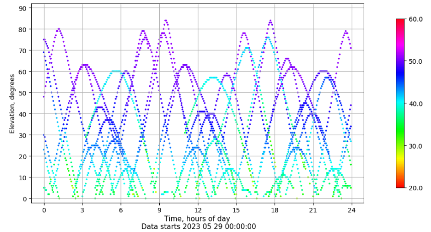
Time-elevation plot for station BCL1. Signal to Noise S1C Data file BCL100ESP_R_2023149.xtr
