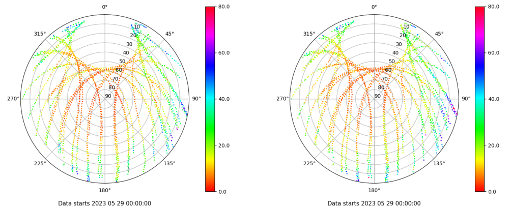
Skyplot for station BCL1. Parameter M1C Data file BCL100ESP_R_2023149.xtr Skyplot for station BCL1. Parameter M2P Data file BCL100ESP_R_2023149.xtr
