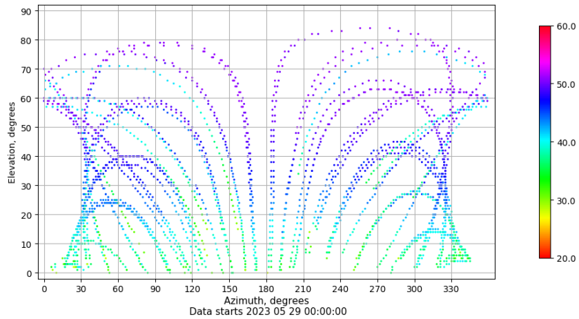
Azimuth-elevation plot for station BCL1. Signal to Noise S1C Data file BCL100ESP_R_2023149.xtr
