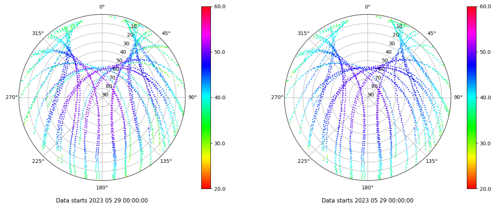
Skyplot for station BCL1. Signal to Noise S1C Data file BCL100ESP_R_2023149.xtr Skyplot for station BCL1. Signal to Noise S2P Data file BCL100ESP_R_2023149.xtr
