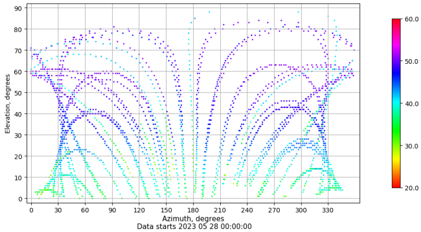
Azimuth-elevation plot for station BCL1. Signal to Noise S1C Data file BCL100ESP_R_2023148.xtr
