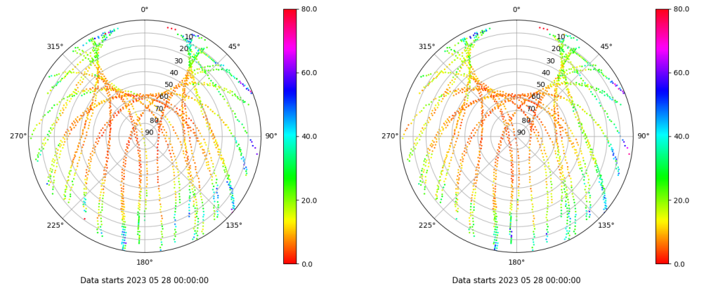
Skyplot for station BCL1. Parameter M1C Data file BCL100ESP_R_2023148.xtr Skyplot for station BCL1. Parameter M2P Data file BCL100ESP_R_2023148.xtr
