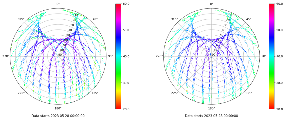
Skyplot for station BCL1. Signal to Noise S1C Data file BCL100ESP_R_2023148.xtr Skyplot for station BCL1. Signal to Noise S2P Data file BCL100ESP_R_2023148.xtr
