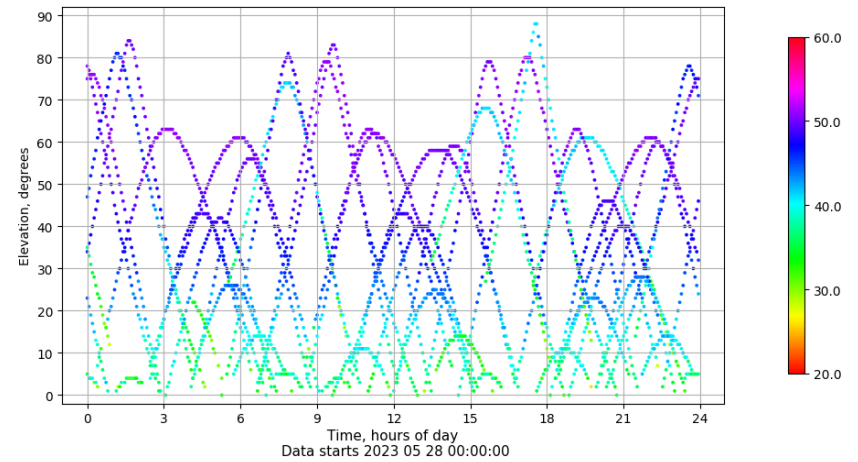
Time-elevation plot for station BCL1. Signal to Noise S1C Data file BCL100ESP_R_2023148.xtr
