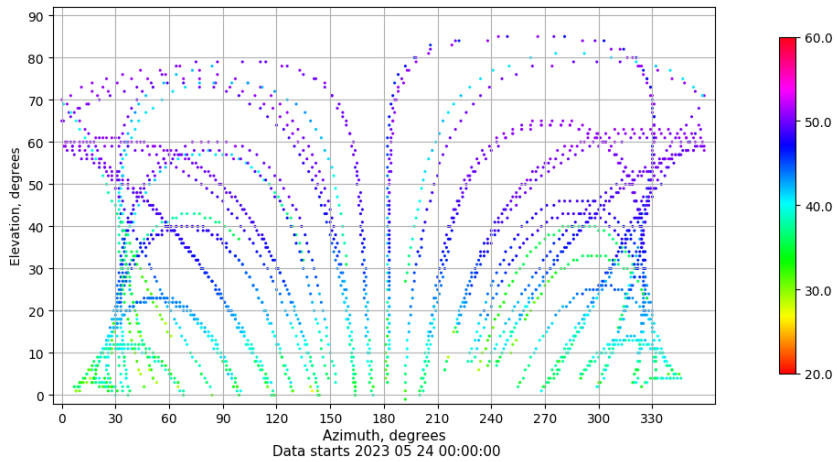
Azimuth-elevation plot for station BCL1. Signal to Noise S1C Data file BCL100ESP_R_2023144.xtr
