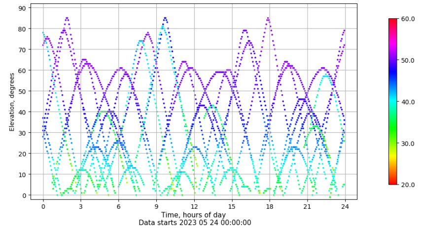
Time-elevation plot for station BCL1. Signal to Noise S1C Data file BCL100ESP_R_2023144.xtr
