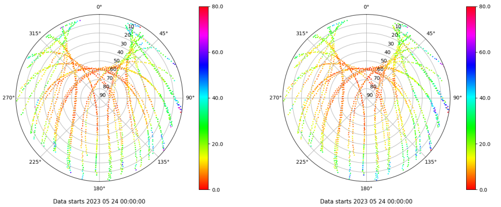
Skyplot for station BCL1. Parameter M1C Data file BCL100ESP_R_2023144.xtr Skyplot for station BCL1. Parameter M2P Data file BCL100ESP_R_2023144.xtr
