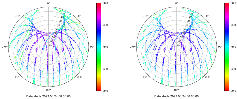
Skyplot for station BCL1. Signal to Noise S1C Data file BCL100ESP_R_2023144.xtr Skyplot for station BCL1. Signal to Noise S2P Data file BCL100ESP_R_2023144.xtr
