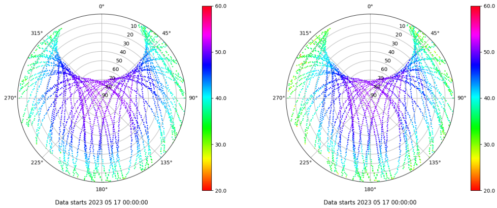
Skyplot for station BCL1. Signal to Noise S1C Data file BCL100ESP_R_2023137.xtr Skyplot for station BCL1. Signal to Noise S2W Data file BCL100ESP_R_2023137.xtr
