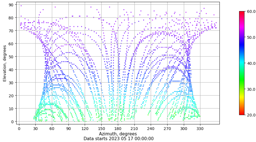
Azimuth-elevation plot for station BCL1. Signal to Noise S1C Data file BCL100ESP_R_2023137.xtr
