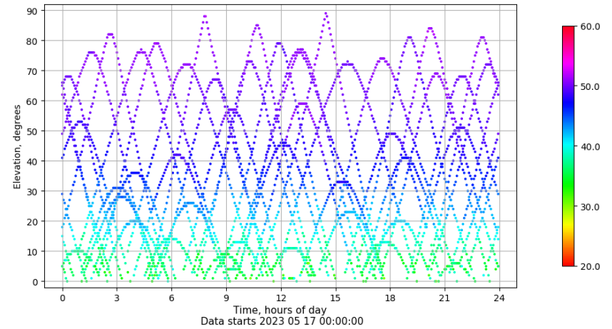
Time-elevation plot for station BCL1. Signal to Noise S1C Data file BCL100ESP_R_2023137.xtr
