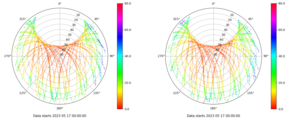
Skyplot for station BCL1. Parameter M1C Data file BCL100ESP_R_2023137.xtr Skyplot for station BCL1. Parameter M2W Data file BCL100ESP_R_2023137.xtr
