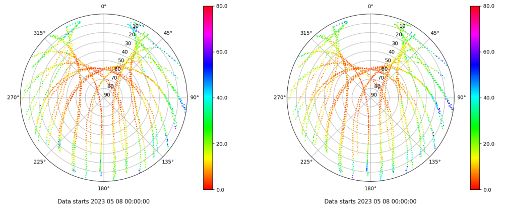
Skyplot for station BCL1. Parameter M1C Data file BCL100ESP_R_2023128.xtr Skyplot for station BCL1. Parameter M2P Data file BCL100ESP_R_2023128.xtr
