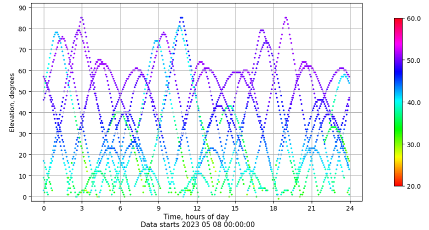
Time-elevation plot for station BCL1. Signal to Noise S1C Data file BCL100ESP_R_2023128.xtr
