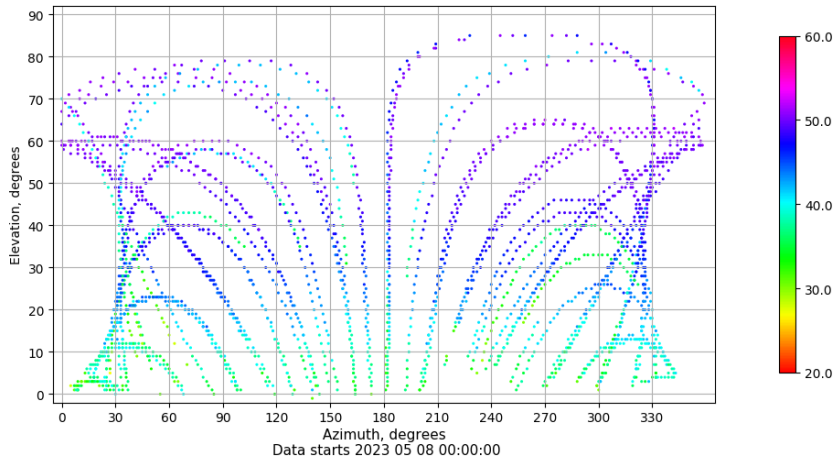
Azimuth-elevation plot for station BCL1. Signal to Noise S1C Data file BCL100ESP_R_2023128.xtr
