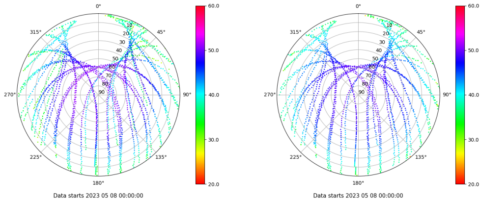
Skyplot for station BCL1. Signal to Noise S1C Data file BCL100ESP_R_2023128.xtr Skyplot for station BCL1. Signal to Noise S2P Data file BCL100ESP_R_2023128.xtr
