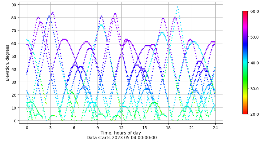
Time-elevation plot for station BCL1. Signal to Noise S1C Data file BCL100ESP_R_2023124.xtr
