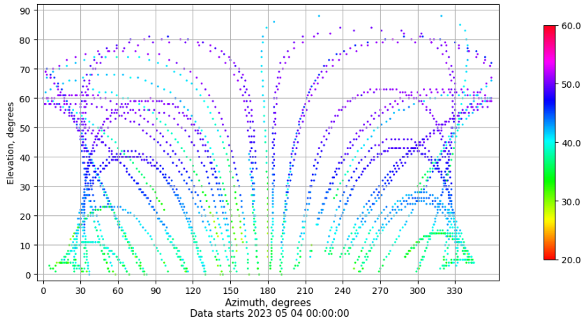
Azimuth-elevation plot for station BCL1. Signal to Noise S1C Data file BCL100ESP_R_2023124.xtr
