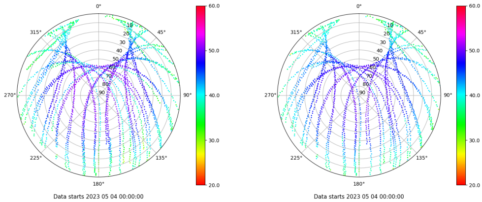
Skyplot for station BCL1. Signal to Noise S1C Data file BCL100ESP_R_2023124.xtr Skyplot for station BCL1. Signal to Noise S2P Data file BCL100ESP_R_2023124.xtr
