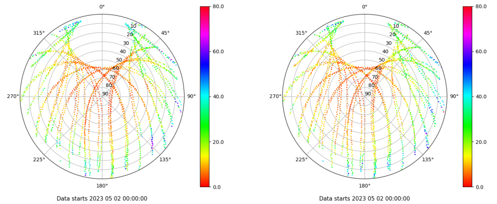
Skyplot for station BCL1. Parameter M1C Data file BCL100ESP_R_2023122.xtr Skyplot for station BCL1. Parameter M2P Data file BCL100ESP_R_2023122.xtr
