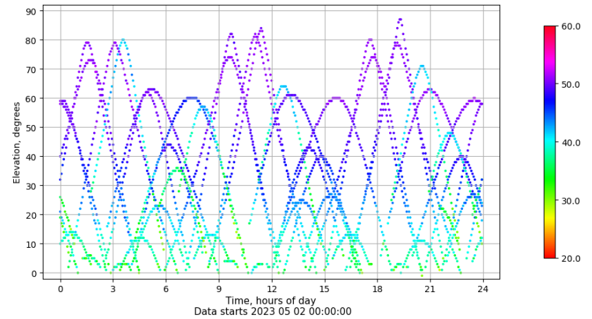
Time-elevation plot for station BCL1. Signal to Noise S1C Data file BCL100ESP_R_2023122.xtr
