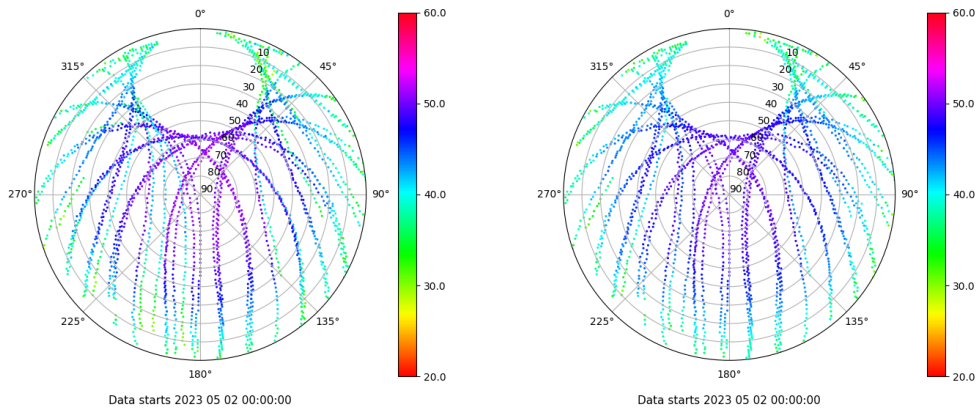
Skyplot for station BCL1. Signal to Noise S1C Data file BCL100ESP_R_2023122.xtr Skyplot for station BCL1. Signal to Noise S2P Data file BCL100ESP_R_2023122.xtr
