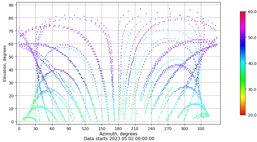
Azimuth-elevation plot for station BCL1. Signal to Noise S1C Data file BCL100ESP_R_2023122.xtr
