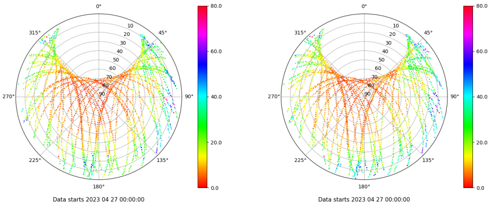
Skyplot for station BCL1. Parameter M1C Data file BCL100ESP_R_2023117.xtr Skyplot for station BCL1. Parameter M2W Data file BCL100ESP_R_2023117.xtr
