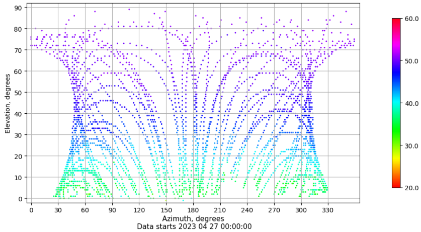
Azimuth-elevation plot for station BCL1. Signal to Noise S1C Data file BCL100ESP_R_2023117.xtr
