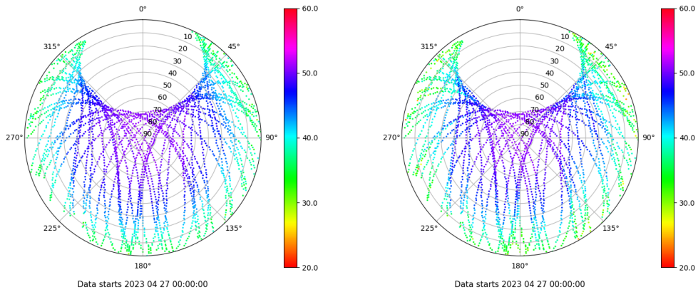
Skyplot for station BCL1. Signal to Noise S1C Data file BCL100ESP_R_2023117.xtr Skyplot for station BCL1. Signal to Noise S2W Data file BCL100ESP_R_2023117.xtr
