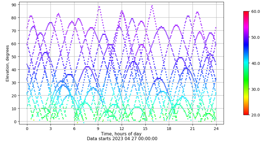
Time-elevation plot for station BCL1. Signal to Noise S1C Data file BCL100ESP_R_2023117.xtr
