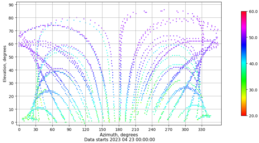
Azimuth-elevation plot for station BCL1. Signal to Noise S1C Data file BCL100ESP_R_2023113.xtr
