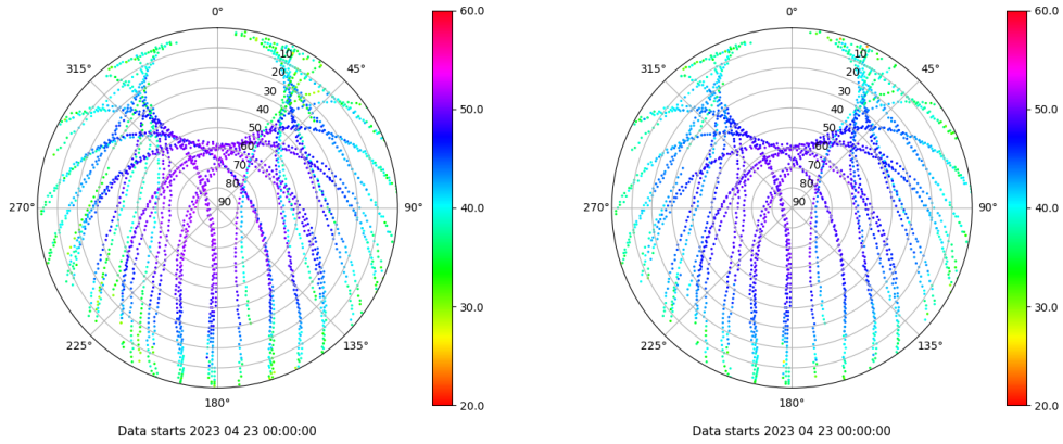
Skyplot for station BCL1. Signal to Noise S1C Data file BCL100ESP_R_2023113.xtr Skyplot for station BCL1. Signal to Noise S2P Data file BCL100ESP_R_2023113.xtr
