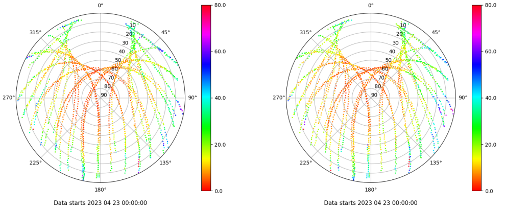
Skyplot for station BCL1. Parameter M1C Data file BCL100ESP_R_2023113.xtr Skyplot for station BCL1. Parameter M2P Data file BCL100ESP_R_2023113.xtr
