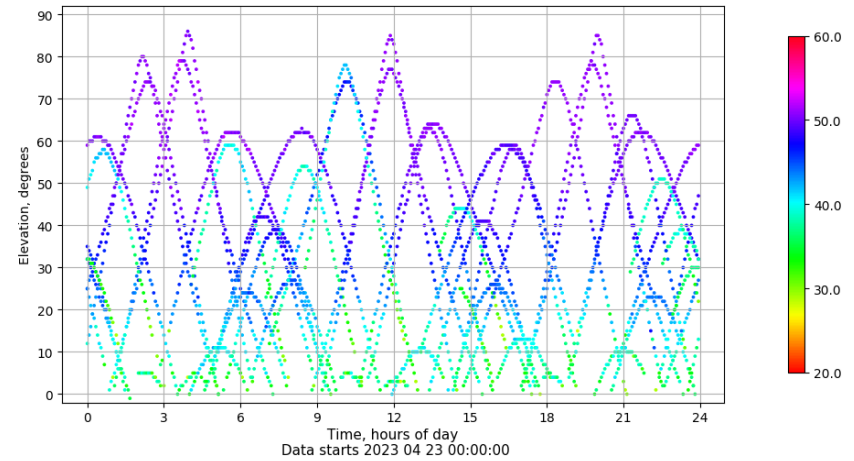
Time-elevation plot for station BCL1. Signal to Noise S1C Data file BCL100ESP_R_2023113.xtr
