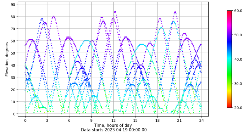
Time-elevation plot for station BCL1. Signal to Noise S1C Data file BCL100ESP_R_2023109.xtr
