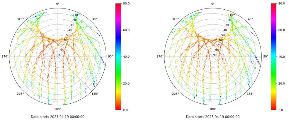
Skyplot for station BCL1. Parameter M1C Data file BCL100ESP_R_2023109.xtr Skyplot for station BCL1. Parameter M2P Data file BCL100ESP_R_2023109.xtr
