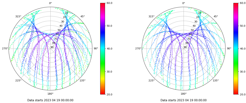
Skyplot for station BCL1. Signal to Noise S1C Data file BCL100ESP_R_2023109.xtr Skyplot for station BCL1. Signal to Noise S2P Data file BCL100ESP_R_2023109.xtr
