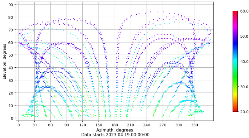
Azimuth-elevation plot for station BCL1. Signal to Noise S1C Data file BCL100ESP_R_2023109.xtr
