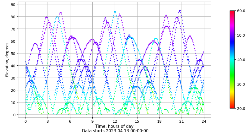
Time-elevation plot for station BCL1. Signal to Noise S1C Data file BCL100ESP_R_2023103.xtr
