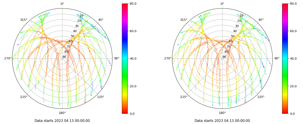
Skyplot for station BCL1. Parameter M1C Data file BCL100ESP_R_2023103.xtr Skyplot for station BCL1. Parameter M2P Data file BCL100ESP_R_2023103.xtr
