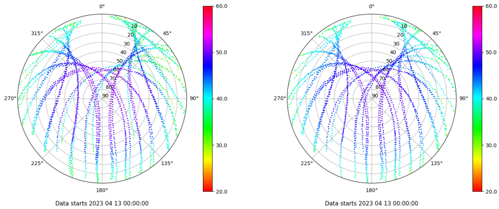
Skyplot for station BCL1. Signal to Noise S1C Data file BCL100ESP_R_2023103.xtr Skyplot for station BCL1. Signal to Noise S2P Data file BCL100ESP_R_2023103.xtr
