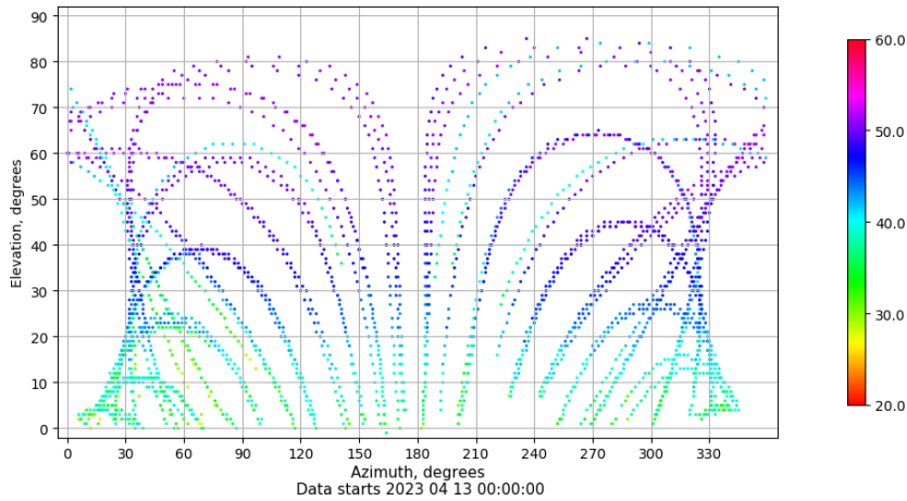
Azimuth-elevation plot for station BCL1. Signal to Noise S1C Data file BCL100ESP_R_2023103.xtr
