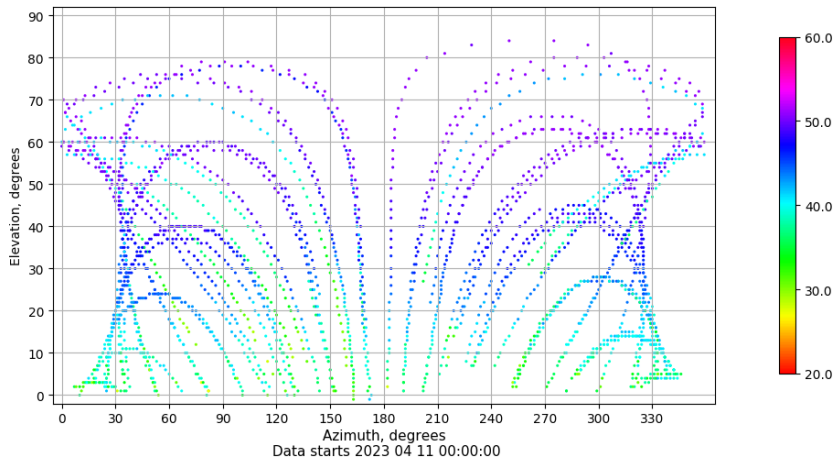
Azimuth-elevation plot for station BCL1. Signal to Noise S1C Data file BCL100ESP_R_2023101.xtr
