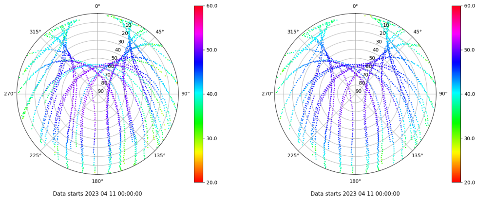
Skyplot for station BCL1. Signal to Noise S1C Data file BCL100ESP_R_2023101.xtr Skyplot for station BCL1. Signal to Noise S2P Data file BCL100ESP_R_2023101.xtr
