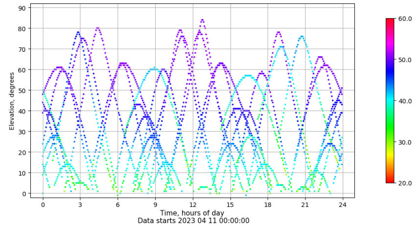
Time-elevation plot for station BCL1. Signal to Noise S1C Data file BCL100ESP_R_2023101.xtr
