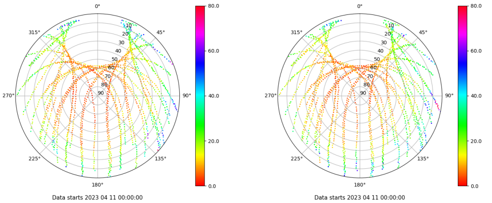
Skyplot for station BCL1. Parameter M1C Data file BCL100ESP_R_2023101.xtr Skyplot for station BCL1. Parameter M2P Data file BCL100ESP_R_2023101.xtr
