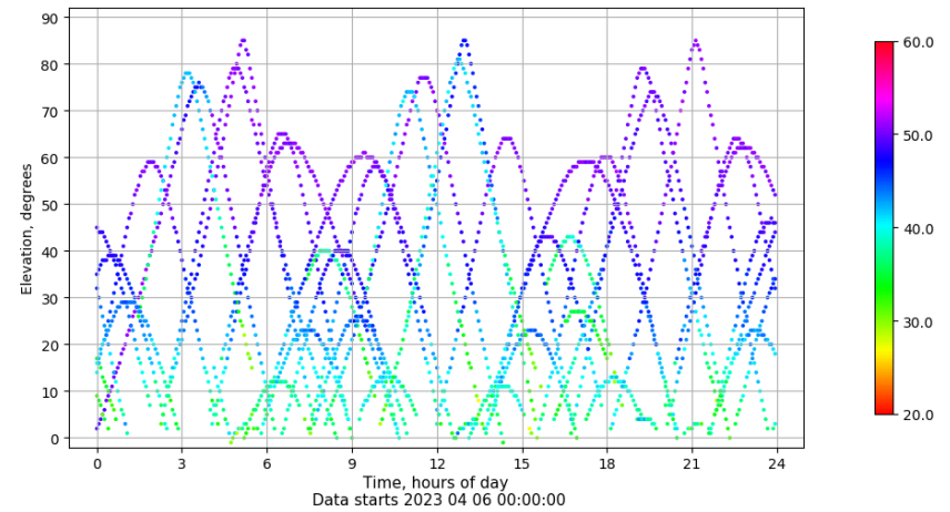
Time-elevation plot for station BCL1. Signal to Noise S1C Data file BCL100ESP_R_2023096.xtr
