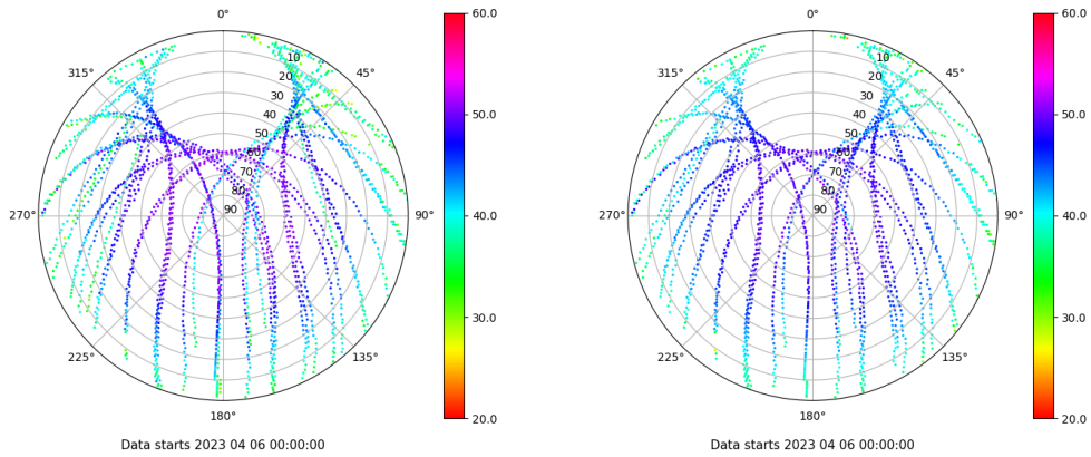
Skyplot for station BCL1. Signal to Noise S1C Data file BCL100ESP_R_2023096.xtr Skyplot for station BCL1. Signal to Noise S2P Data file BCL100ESP_R_2023096.xtr
