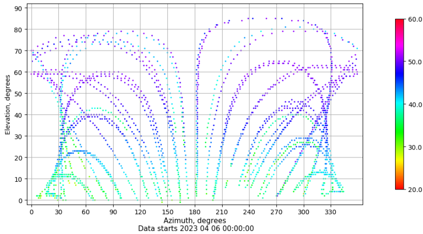
Azimuth-elevation plot for station BCL1. Signal to Noise S1C Data file BCL100ESP_R_2023096.xtr
