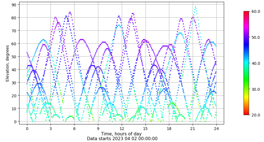
Time-elevation plot for station BCL1. Signal to Noise S1C Data file BCL100ESP_R_2023092.xtr
