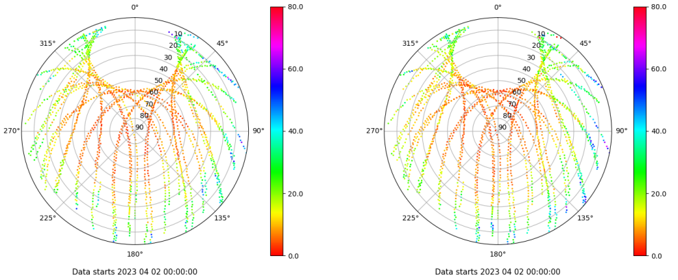
Skyplot for station BCL1. Parameter M1C Data file BCL100ESP_R_2023092.xtr Skyplot for station BCL1. Parameter M2P Data file BCL100ESP_R_2023092.xtr
