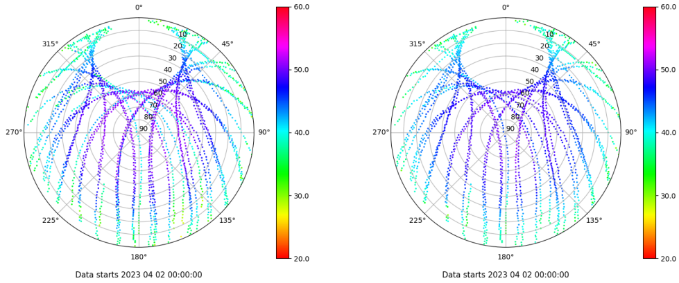
Skyplot for station BCL1. Signal to Noise S1C Data file BCL100ESP_R_2023092.xtr Skyplot for station BCL1. Signal to Noise S2P Data file BCL100ESP_R_2023092.xtr
