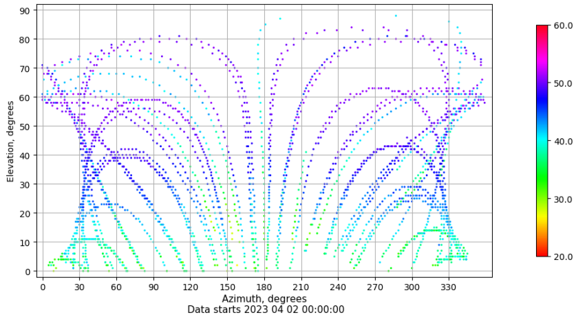
Azimuth-elevation plot for station BCL1. Signal to Noise S1C Data file BCL100ESP_R_2023092.xtr
