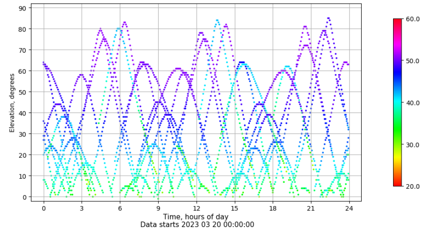
Time-elevation plot for station BCL1. Signal to Noise S1C Data file BCL100ESP_R_2023079.xtr
