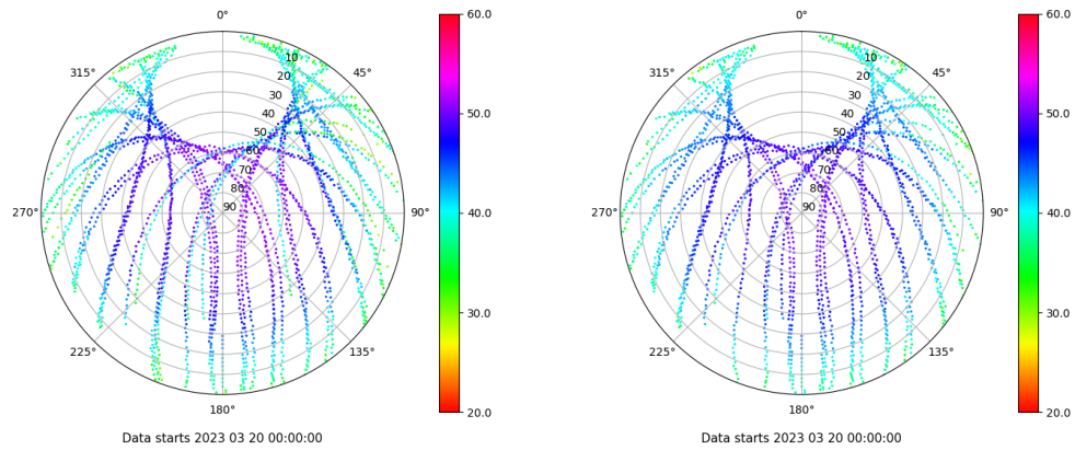
Skyplot for station BCL1. Signal to Noise S1C Data file BCL100ESP_R_2023079.xtr Skyplot for station BCL1. Signal to Noise S2P Data file BCL100ESP_R_2023079.xtr
