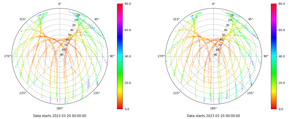
Skyplot for station BCL1. Parameter M1C Data file BCL100ESP_R_2023079.xtr Skyplot for station BCL1. Parameter M2P Data file BCL100ESP_R_2023079.xtr
