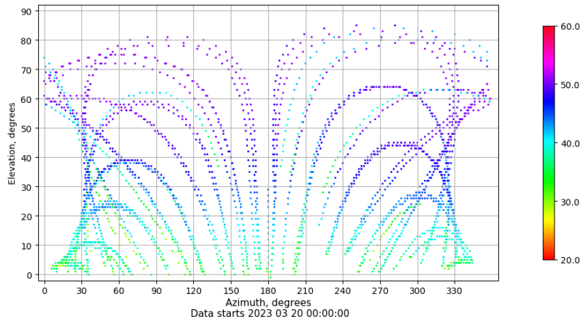
Azimuth-elevation plot for station BCL1. Signal to Noise S1C Data file BCL100ESP_R_2023079.xtr
