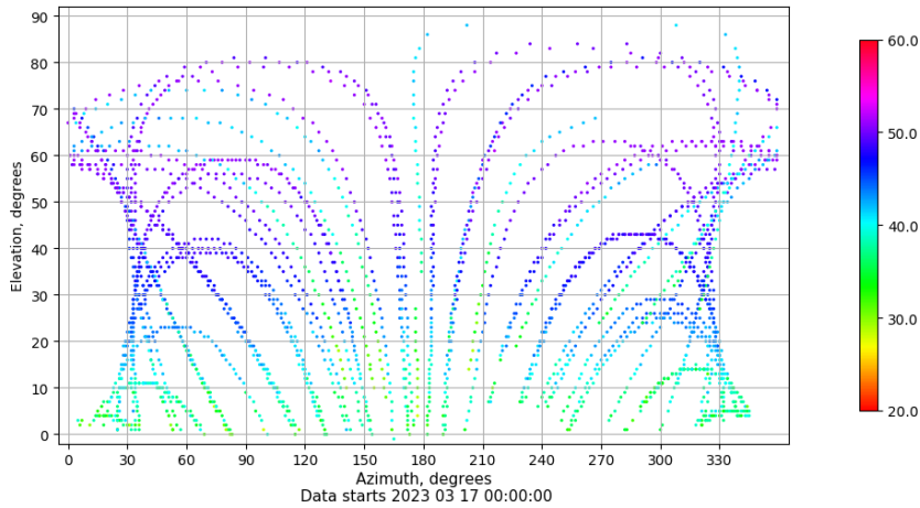
Azimuth-elevation plot for station BCL1. Signal to Noise S1C Data file BCL100ESP_R_2023076.xtr
