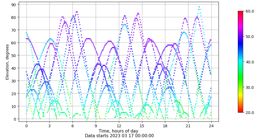
Time-elevation plot for station BCL1. Signal to Noise S1C Data file BCL100ESP_R_2023076.xtr
