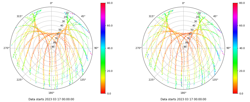
Skyplot for station BCL1. Parameter M1C Data file BCL100ESP_R_2023076.xtr Skyplot for station BCL1. Parameter M2P Data file BCL100ESP_R_2023076.xtr
