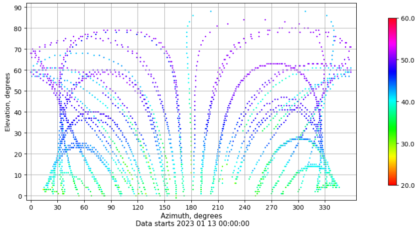
Azimuth-elevation plot for station BCL1. Signal to Noise S1C Data file BCL100ESP_R_2023013.xtr
