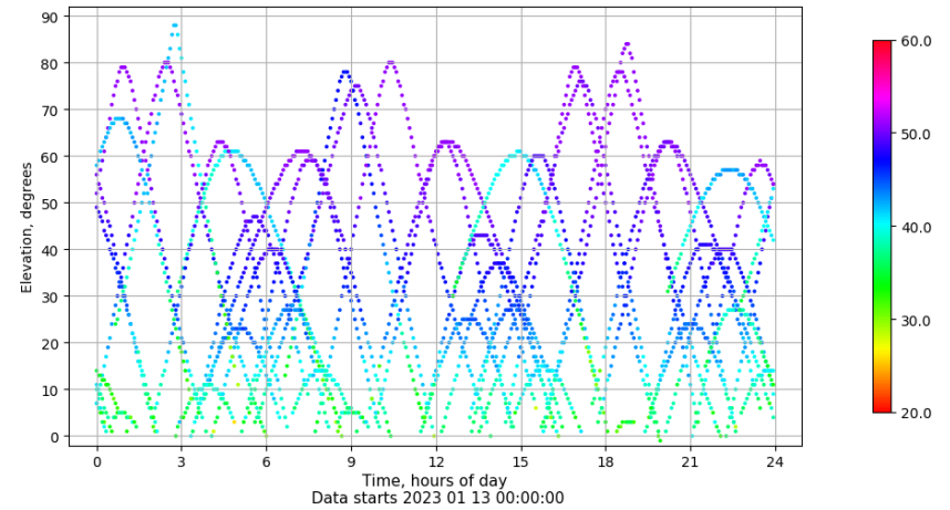
Time-elevation plot for station BCL1. Signal to Noise S1C Data file BCL100ESP_R_2023013.xtr
