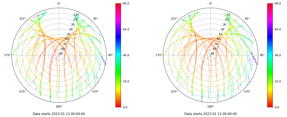
Skyplot for station BCL1. Parameter M1C Data file BCL100ESP_R_2023013.xtr Skyplot for station BCL1. Parameter M2P Data file BCL100ESP_R_2023013.xtr
