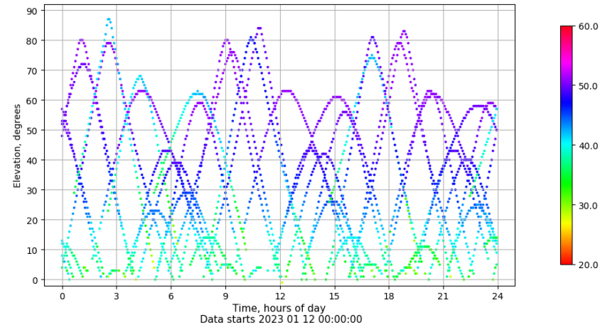
Time-elevation plot for station BCL1. Signal to Noise S1C Data file BCL100ESP_R_2023012.xtr
