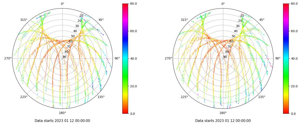
Skyplot for station BCL1. Parameter M1C Data file BCL100ESP_R_2023012.xtr Skyplot for station BCL1. Parameter M2P Data file BCL100ESP_R_2023012.xtr
