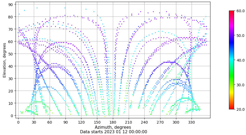
Azimuth-elevation plot for station BCL1. Signal to Noise S1C Data file BCL100ESP_R_2023012.xtr
