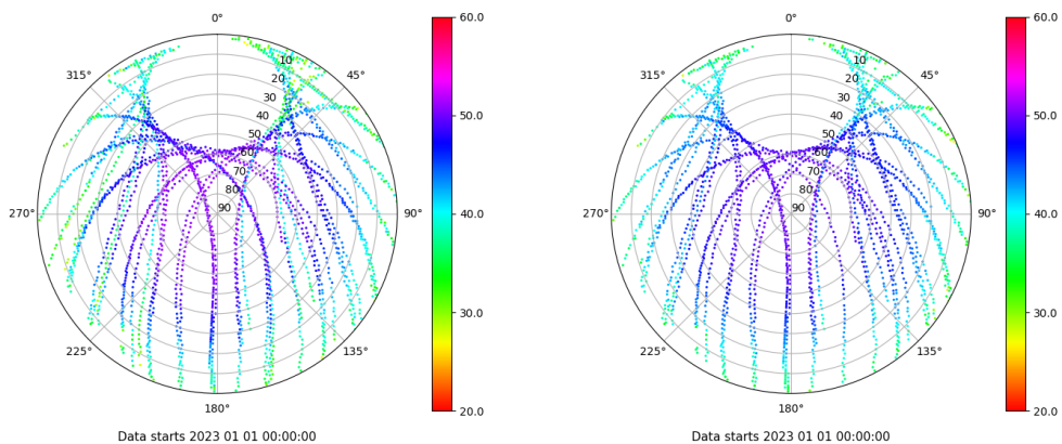
Skyplot for station BCL1. Signal to Noise S1C Data file BCL100ESP_R_2023001.xtr Skyplot for station BCL1. Signal to Noise S2P Data file BCL100ESP_R_2023001.xtr
