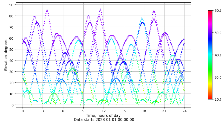
Time-elevation plot for station BCL1. Signal to Noise S1C Data file BCL100ESP_R_2023001.xtr
