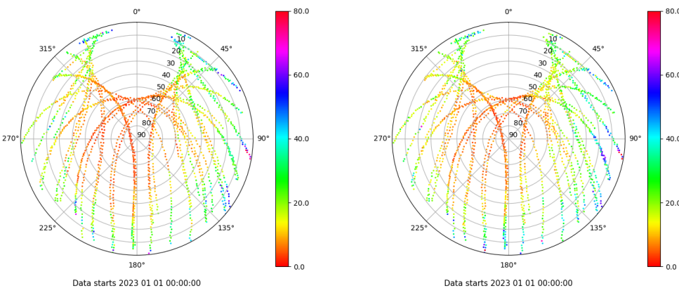
Skyplot for station BCL1. Parameter M1C Data file BCL100ESP_R_2023001.xtr Skyplot for station BCL1. Parameter M2P Data file BCL100ESP_R_2023001.xtr
