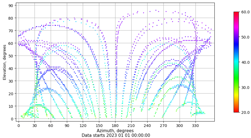
Azimuth-elevation plot for station BCL1. Signal to Noise S1C Data file BCL100ESP_R_2023001.xtr
