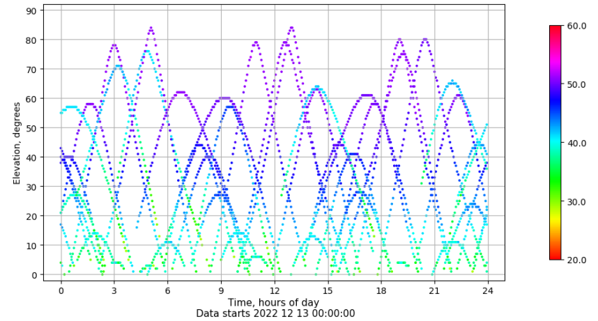
Time-elevation plot for station BCL1. Signal to Noise S1C Data file BCL100ESP_R_2022347.xtr
