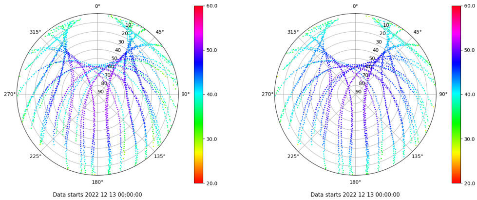
Skyplot for station BCL1. Signal to Noise S1C Data file BCL100ESP_R_2022347.xtr Skyplot for station BCL1. Signal to Noise S2P Data file BCL100ESP_R_2022347.xtr
