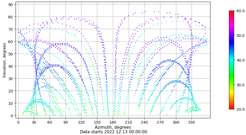
Azimuth-elevation plot for station BCL1. Signal to Noise S1C Data file BCL100ESP_R_2022347.xtr
