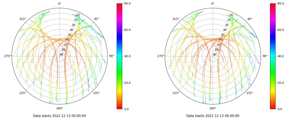
Skyplot for station BCL1. Parameter M1C Data file BCL100ESP_R_2022347.xtr Skyplot for station BCL1. Parameter M2P Data file BCL100ESP_R_2022347.xtr
