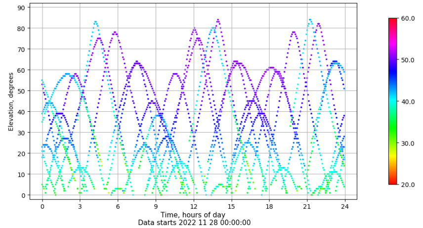
Time-elevation plot for station BCL1. Signal to Noise S1C Data file BCL100ESP_R_2022332.xtr
