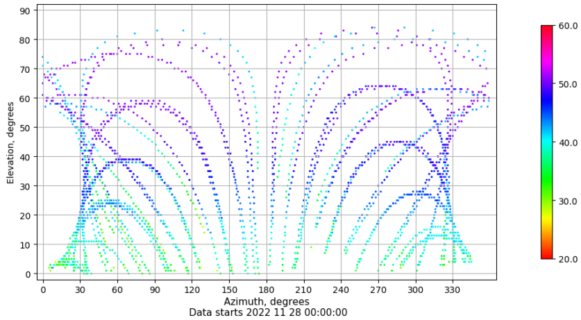
Azimuth-elevation plot for station BCL1. Signal to Noise S1C Data file BCL100ESP_R_2022332.xtr
