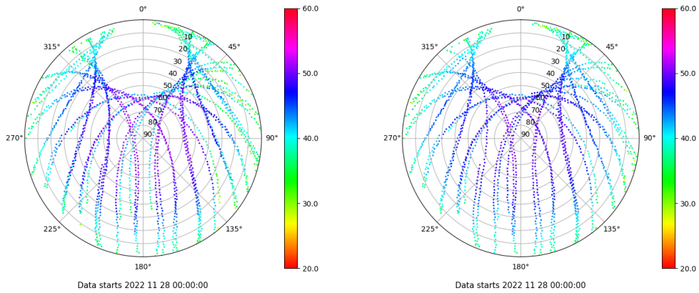
Skyplot for station BCL1. Signal to Noise S1C Data file BCL100ESP_R_2022332.xtr Skyplot for station BCL1. Signal to Noise S2P Data file BCL100ESP_R_2022332.xtr
