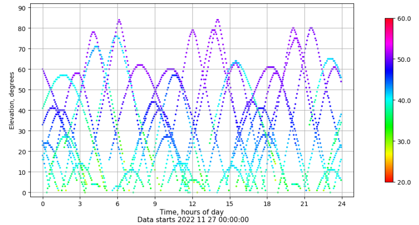
Time-elevation plot for station BCL1. Signal to Noise S1C Data file BCL100ESP_R_2022331.xtr
