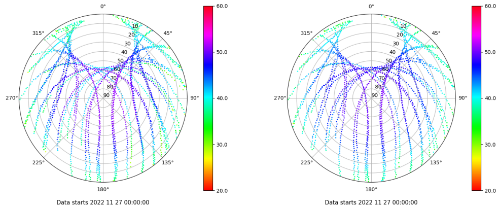
Skyplot for station BCL1. Signal to Noise S1C Data file BCL100ESP_R_2022331.xtr Skyplot for station BCL1. Signal to Noise S2P Data file BCL100ESP_R_2022331.xtr
