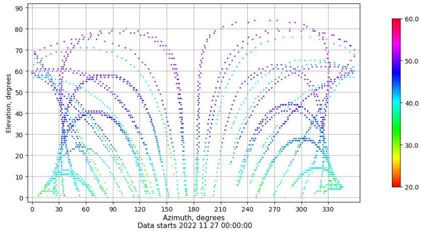
Azimuth-elevation plot for station BCL1. Signal to Noise S1C Data file BCL100ESP_R_2022331.xtr
