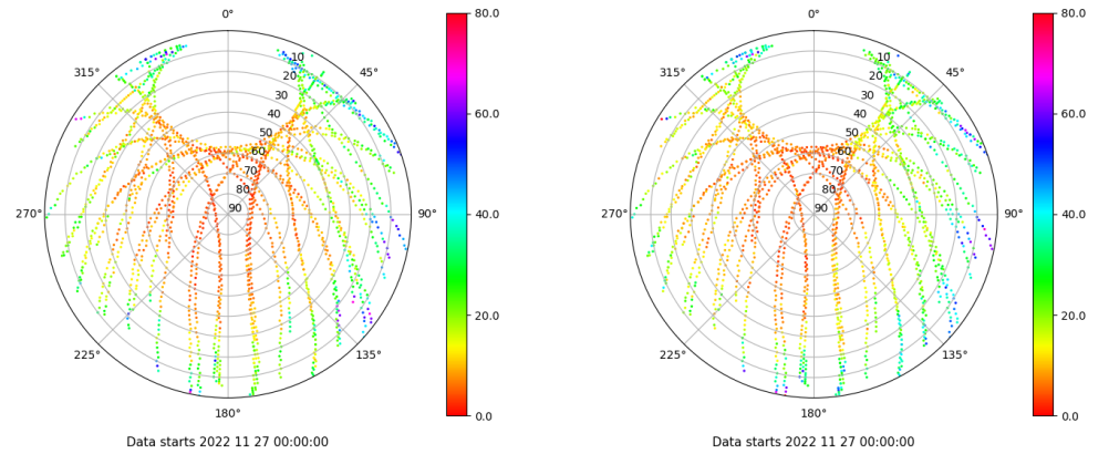
Skyplot for station BCL1. Parameter M1C Data file BCL100ESP_R_2022331.xtr Skyplot for station BCL1. Parameter M2P Data file BCL100ESP_R_2022331.xtr
