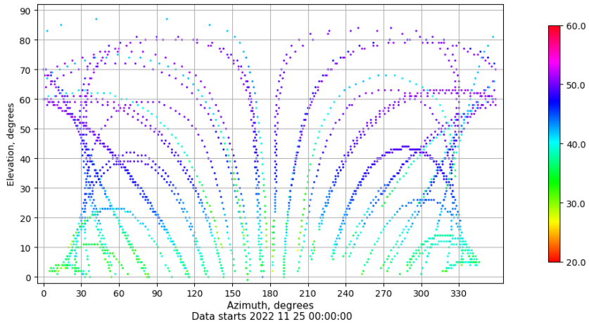
Azimuth-elevation plot for station BCL1. Signal to Noise S1C Data file BCL100ESP_R_2022329.xtr
