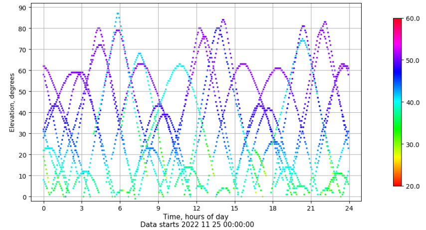
Time-elevation plot for station BCL1. Signal to Noise S1C Data file BCL100ESP_R_2022329.xtr
