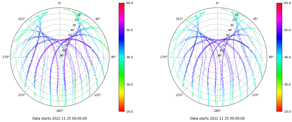
Skyplot for station BCL1. Signal to Noise S1C Data file BCL100ESP_R_2022329.xtr Skyplot for station BCL1. Signal to Noise S2P Data file BCL100ESP_R_2022329.xtr
