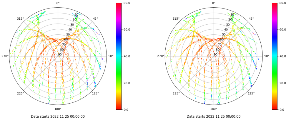
Skyplot for station BCL1. Parameter M1C Data file BCL100ESP_R_2022329.xtr Skyplot for station BCL1. Parameter M2P Data file BCL100ESP_R_2022329.xtr
