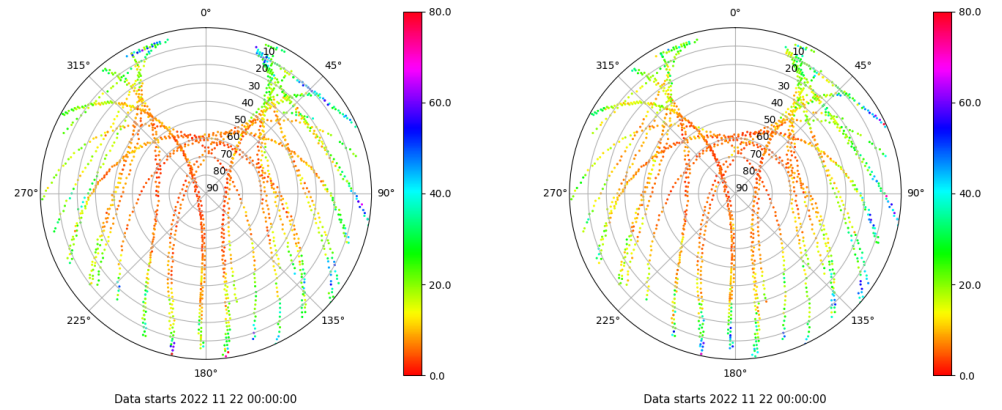
Skyplot for station BCL1. Parameter M1C Data file BCL100ESP_R_2022326.xtr Skyplot for station BCL1. Parameter M2P Data file BCL100ESP_R_2022326.xtr
