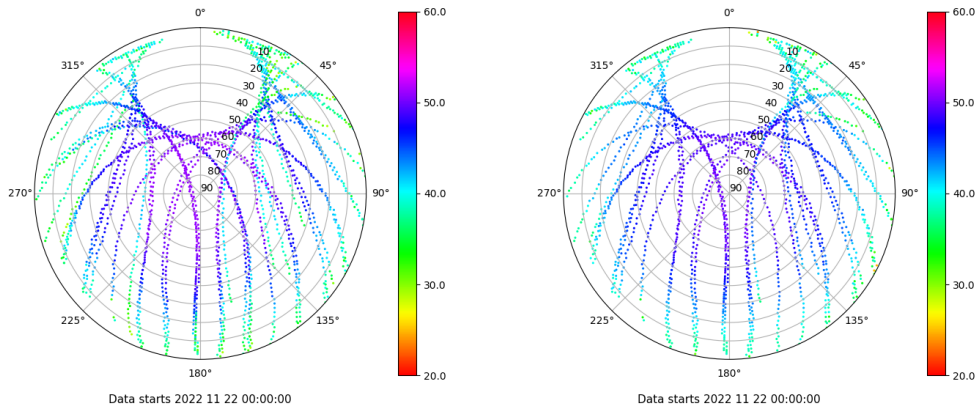
Skyplot for station BCL1. Signal to Noise S1C Data file BCL100ESP_R_2022326.xtr Skyplot for station BCL1. Signal to Noise S2P Data file BCL100ESP_R_2022326.xtr
