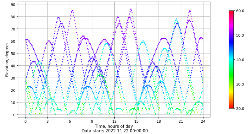
Time-elevation plot for station BCL1. Signal to Noise S1C Data file BCL100ESP_R_2022326.xtr
