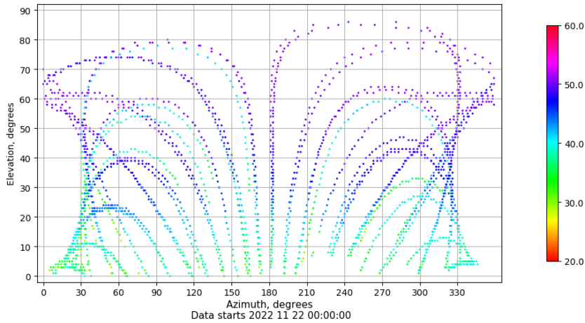
Azimuth-elevation plot for station BCL1. Signal to Noise S1C Data file BCL100ESP_R_2022326.xtr
