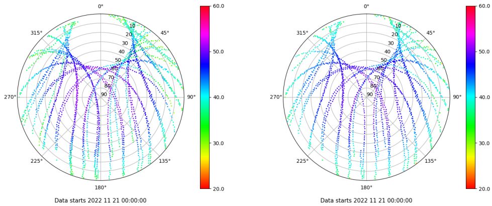
Skyplot for station BCL1. Signal to Noise S1C Data file BCL100ESP_R_2022325.xtr Skyplot for station BCL1. Signal to Noise S2P Data file BCL100ESP_R_2022325.xtr
