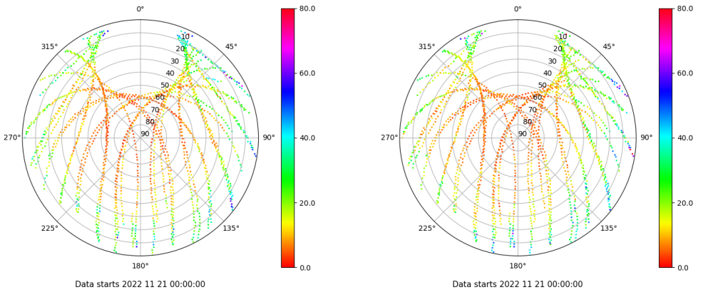
Skyplot for station BCL1. Parameter M1C Data file BCL100ESP_R_2022325.xtr Skyplot for station BCL1. Parameter M2P Data file BCL100ESP_R_2022325.xtr
