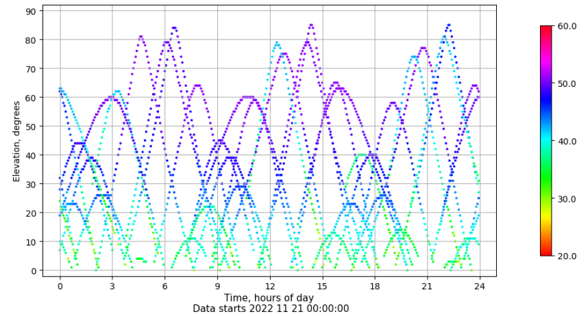
Time-elevation plot for station BCL1. Signal to Noise S1C Data file BCL100ESP_R_2022325.xtr
