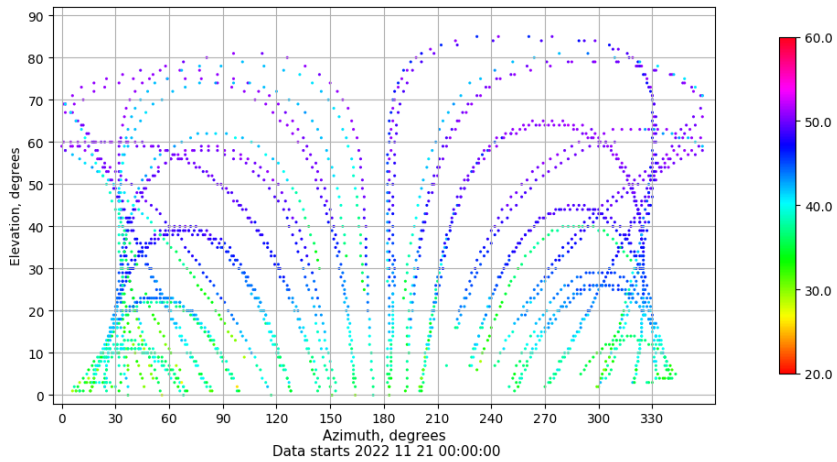
Azimuth-elevation plot for station BCL1. Signal to Noise S1C Data file BCL100ESP_R_2022325.xtr
