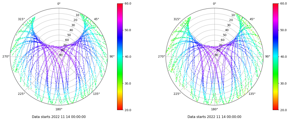
Skyplot for station BCL1. Signal to Noise S1C Data file BCL100ESP_R_2022318.xtr Skyplot for station BCL1. Signal to Noise S2W Data file BCL100ESP_R_2022318.xtr
