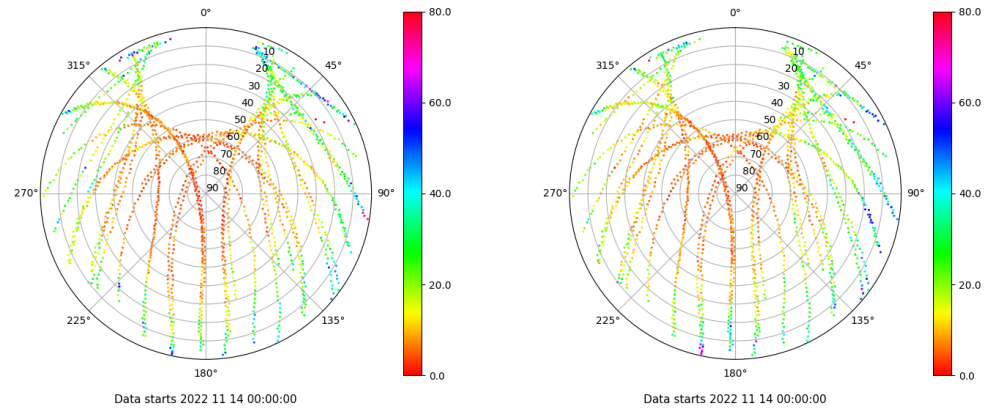
Skyplot for station BCL1. Parameter M1C Data file BCL100ESP_R_2022318.xtr Skyplot for station BCL1. Parameter M2P Data file BCL100ESP_R_2022318.xtr
