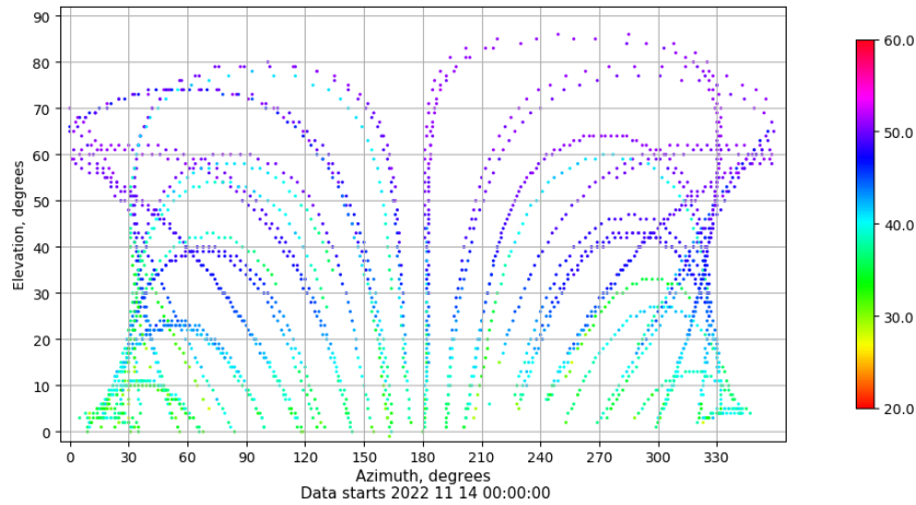
Azimuth-elevation plot for station BCL1. Signal to Noise S1C Data file BCL100ESP_R_2022318.xtr
