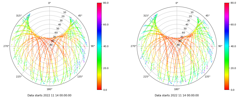
Skyplot for station BCL1. Parameter M1C Data file BCL100ESP_R_2022318.xtr Skyplot for station BCL1. Parameter M2W Data file BCL100ESP_R_2022318.xtr
