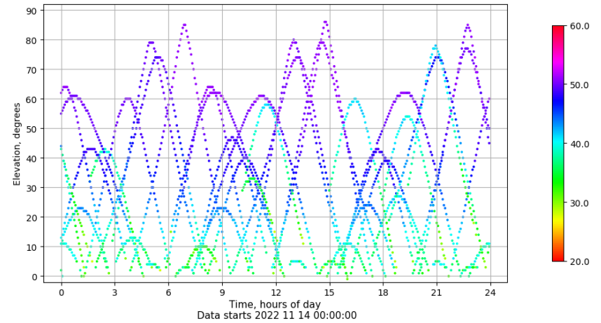
Time-elevation plot for station BCL1. Signal to Noise S1C Data file BCL100ESP_R_2022318.xtr
