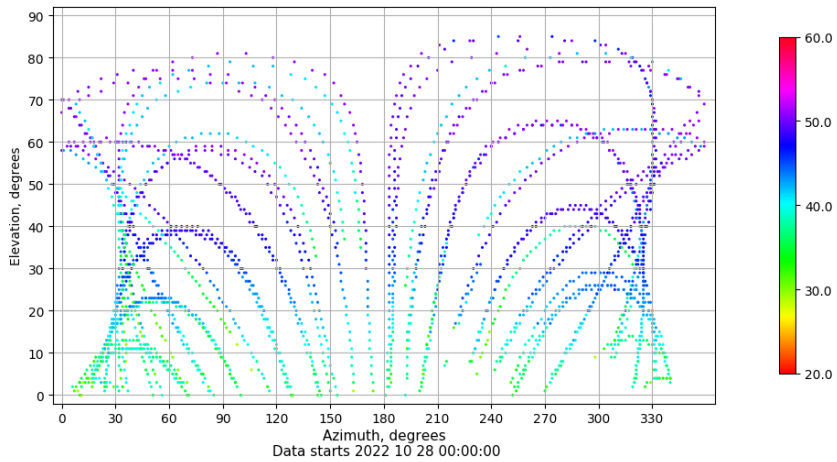
Azimuth-elevation plot for station BCL1. Signal to Noise S1C Data file BCL100ESP_R_2022301.xtr
