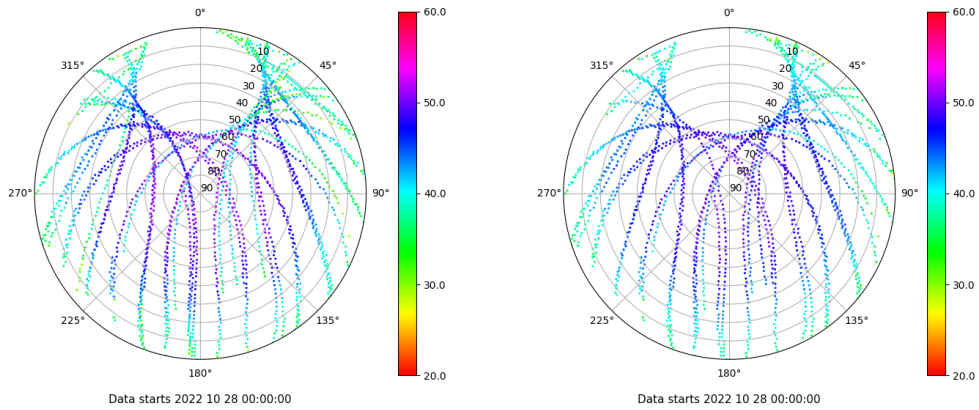
Skyplot for station BCL1. Signal to Noise S1C Data file BCL100ESP_R_2022301.xtr Skyplot for station BCL1. Signal to Noise S2P Data file BCL100ESP_R_2022301.xtr
