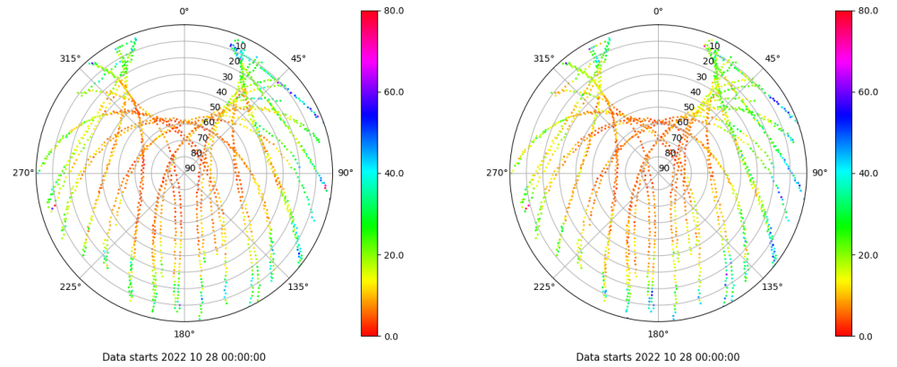
Skyplot for station BCL1. Parameter M1C Data file BCL100ESP_R_2022301.xtr Skyplot for station BCL1. Parameter M2P Data file BCL100ESP_R_2022301.xtr
