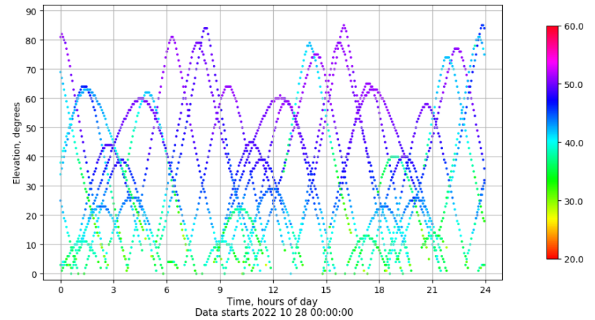
Time-elevation plot for station BCL1. Signal to Noise S1C Data file BCL100ESP_R_2022301.xtr
