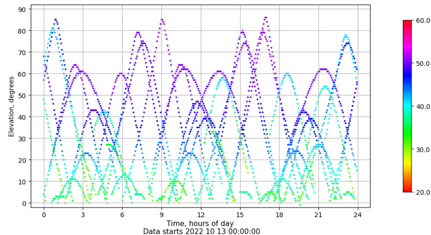
Time-elevation plot for station BCL1. Signal to Noise S1C Data file BCL100ESP_R_2022286.xtr
