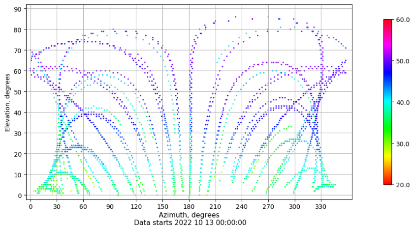
Azimuth-elevation plot for station BCL1. Signal to Noise S1C Data file BCL100ESP_R_2022286.xtr
