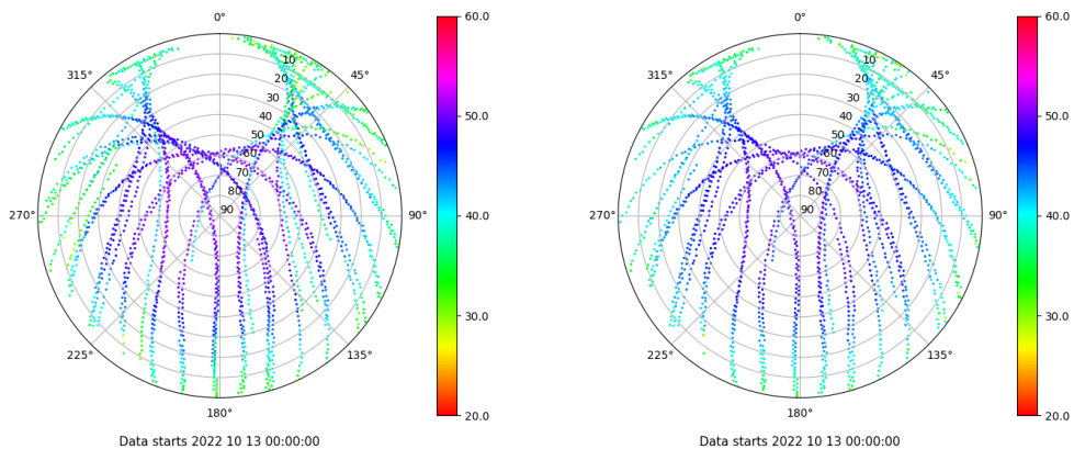
Skyplot for station BCL1. Signal to Noise S1C Data file BCL100ESP_R_2022286.xtr Skyplot for station BCL1. Signal to Noise S2P Data file BCL100ESP_R_2022286.xtr
