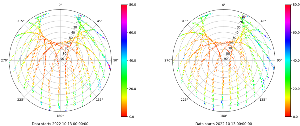
Skyplot for station BCL1. Parameter M1C Data file BCL100ESP_R_2022286.xtr Skyplot for station BCL1. Parameter M2P Data file BCL100ESP_R_2022286.xtr
