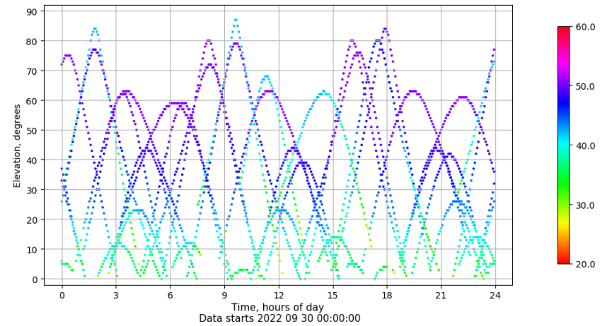
Time-elevation plot for station BCL1. Signal to Noise S1C Data file BCL100ESP_R_2022273.xtr
