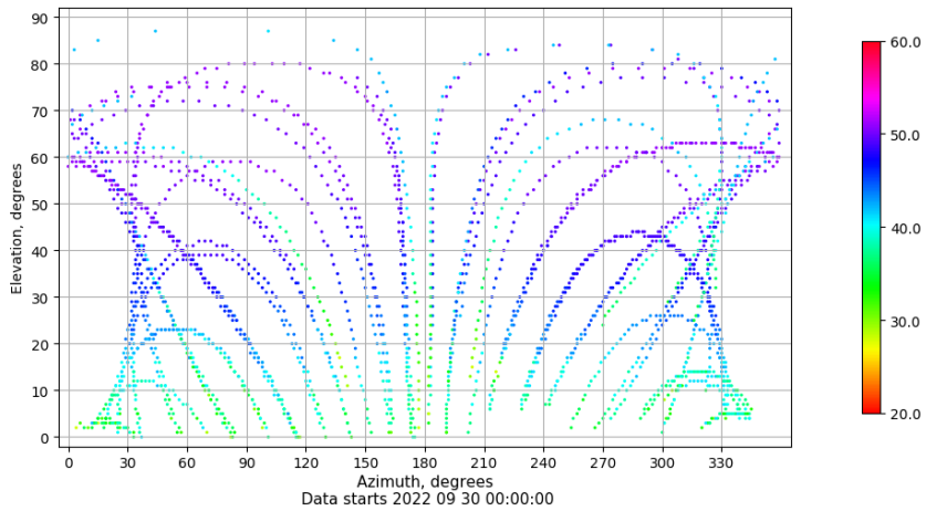
Azimuth-elevation plot for station BCL1. Signal to Noise S1C Data file BCL100ESP_R_2022273.xtr
