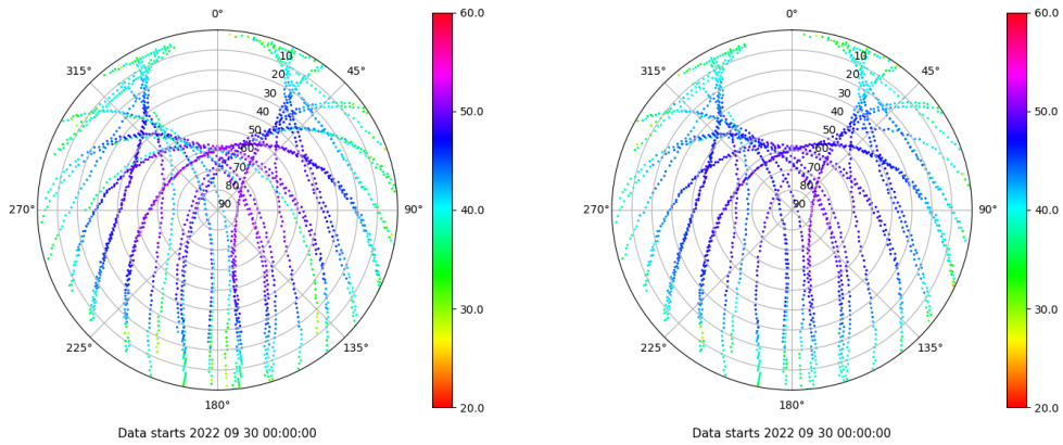
Skyplot for station BCL1. Signal to Noise S1C Data file BCL100ESP_R_2022273.xtr Skyplot for station BCL1. Signal to Noise S2P Data file BCL100ESP_R_2022273.xtr
