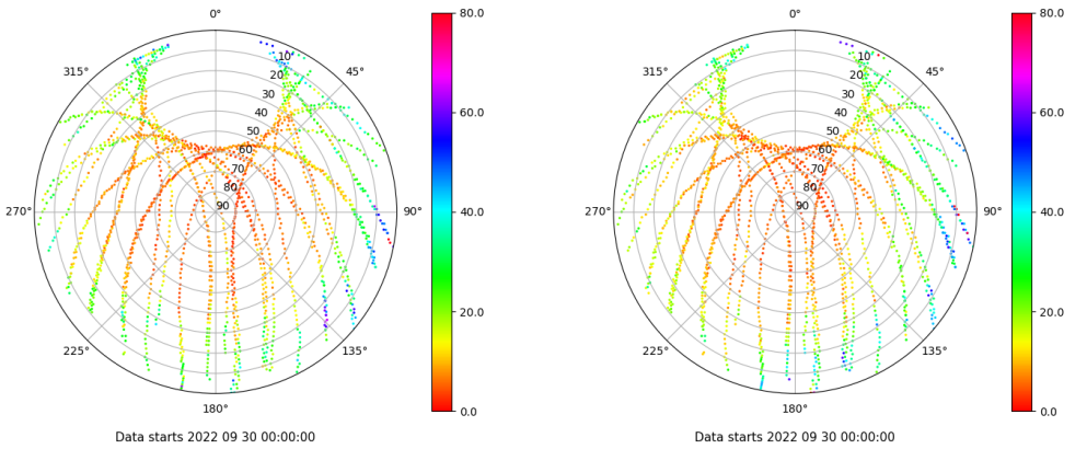
Skyplot for station BCL1. Parameter M1C Data file BCL100ESP_R_2022273.xtr Skyplot for station BCL1. Parameter M2P Data file BCL100ESP_R_2022273.xtr
