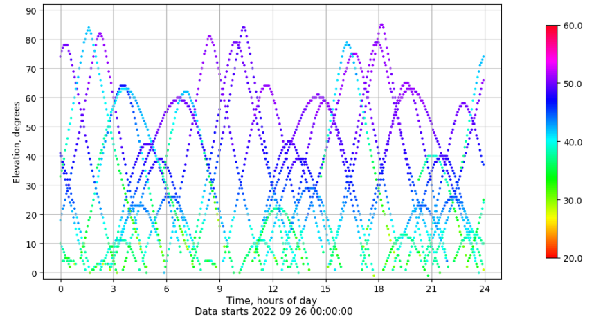
Time-elevation plot for station BCL1. Signal to Noise S1C Data file BCL100ESP_R_2022269.xtr
