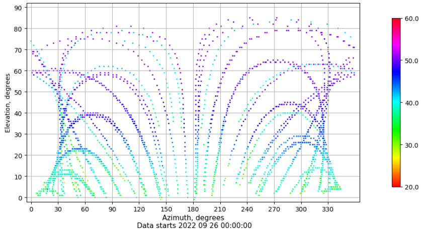
Azimuth-elevation plot for station BCL1. Signal to Noise S1C Data file BCL100ESP_R_2022269.xtr
