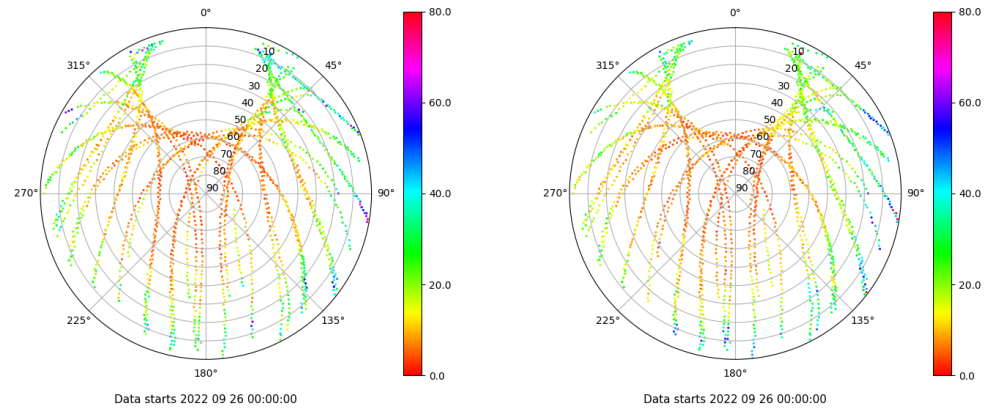
Skyplot for station BCL1. Parameter M1C Data file BCL100ESP_R_2022269.xtr Skyplot for station BCL1. Parameter M2P Data file BCL100ESP_R_2022269.xtr
