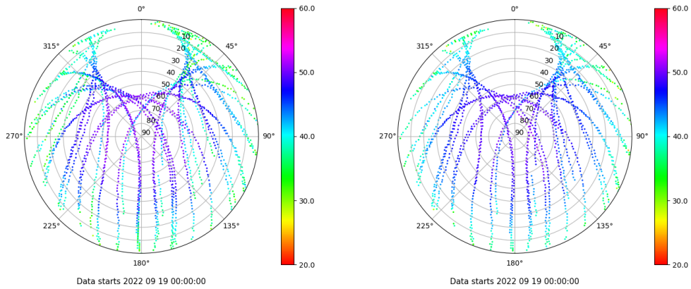
Skyplot for station BCL1. Signal to Noise S1C Data file BCL100ESP_R_2022262.xtr Skyplot for station BCL1. Signal to Noise S2P Data file BCL100ESP_R_2022262.xtr
