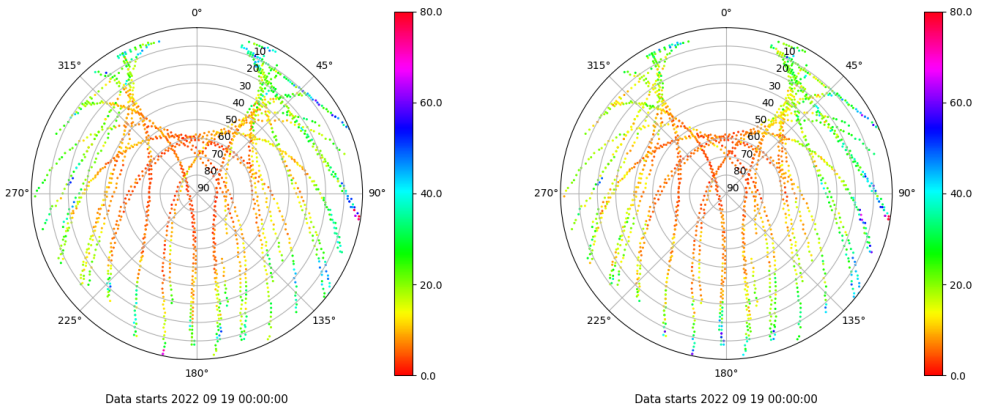
Skyplot for station BCL1. Parameter M1C Data file BCL100ESP_R_2022262.xtr Skyplot for station BCL1. Parameter M2P Data file BCL100ESP_R_2022262.xtr
