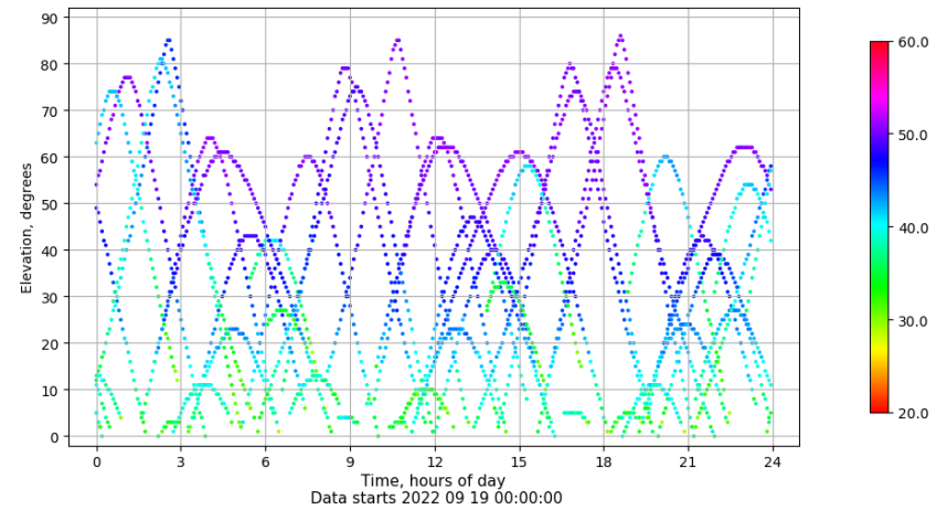
Time-elevation plot for station BCL1. Signal to Noise S1C Data file BCL100ESP_R_2022262.xtr
