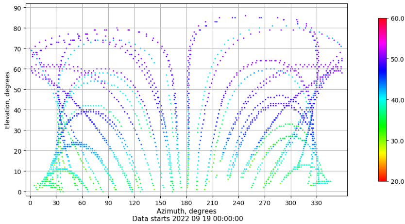
Azimuth-elevation plot for station BCL1. Signal to Noise S1C Data file BCL100ESP_R_2022262.xtr
