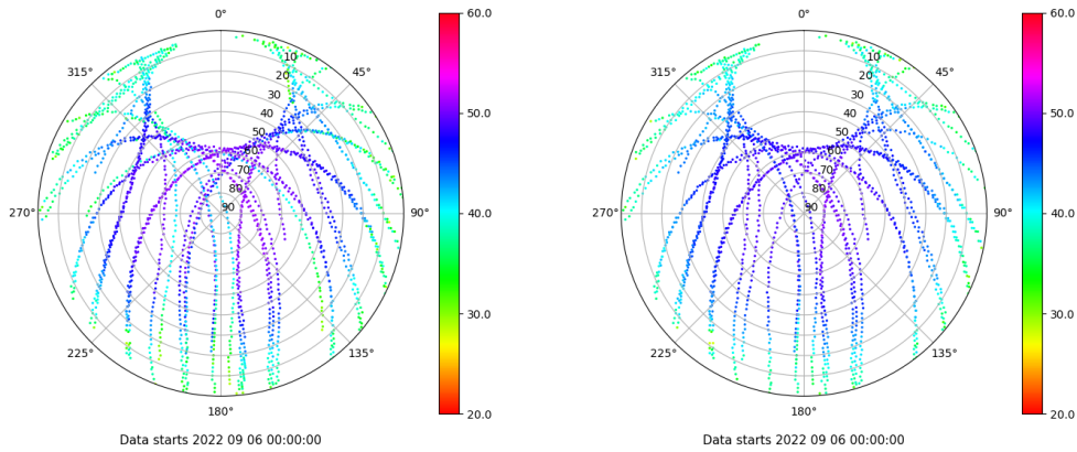
Skyplot for station BCL1. Signal to Noise S1C Data file BCL100ESP_R_2022249.xtr Skyplot for station BCL1. Signal to Noise S2P Data file BCL100ESP_R_2022249.xtr
