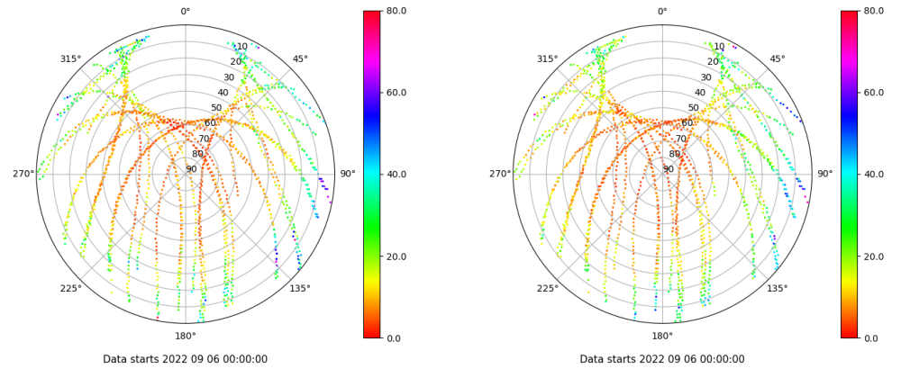
Skyplot for station BCL1. Parameter M1C Data file BCL100ESP_R_2022249.xtr Skyplot for station BCL1. Parameter M2P Data file BCL100ESP_R_2022249.xtr
