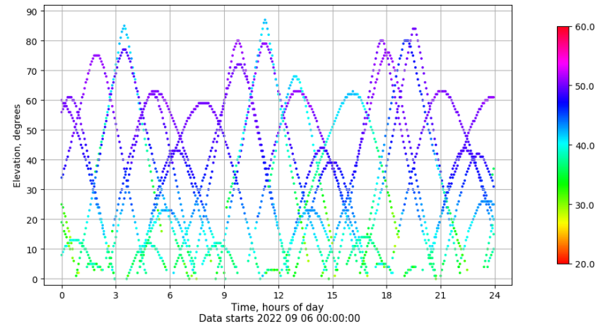
Time-elevation plot for station BCL1. Signal to Noise S1C Data file BCL100ESP_R_2022249.xtr
