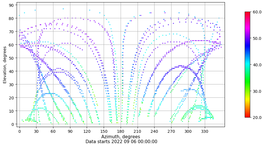
Azimuth-elevation plot for station BCL1. Signal to Noise S1C Data file BCL100ESP_R_2022249.xtr
