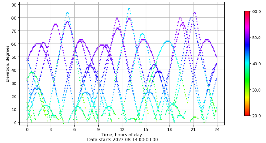
Time-elevation plot for station BCL1. Signal to Noise S1C Data file BCL100ESP_R_2022225.xtr
