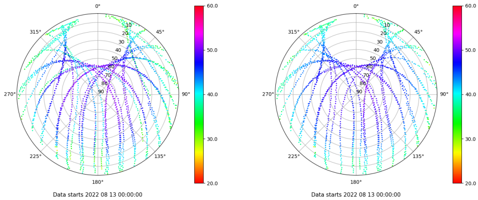
Skyplot for station BCL1. Signal to Noise S1C Data file BCL100ESP_R_2022225.xtr Skyplot for station BCL1. Signal to Noise S2P Data file BCL100ESP_R_2022225.xtr
