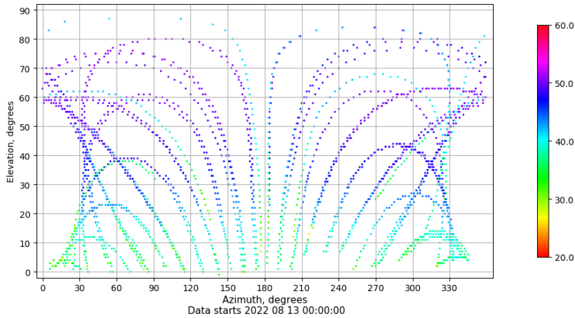
Azimuth-elevation plot for station BCL1. Signal to Noise S1C Data file BCL100ESP_R_2022225.xtr
