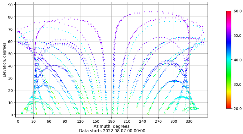
Azimuth-elevation plot for station BCL1. Signal to Noise S1C Data file BCL100ESP_R_2022219.xtr
