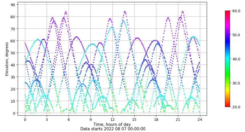
Time-elevation plot for station BCL1. Signal to Noise S1C Data file BCL100ESP_R_2022219.xtr
