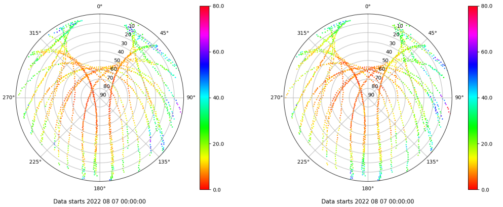
Skyplot for station BCL1. Parameter M1C Data file BCL100ESP_R_2022219.xtr Skyplot for station BCL1. Parameter M2P Data file BCL100ESP_R_2022219.xtr
