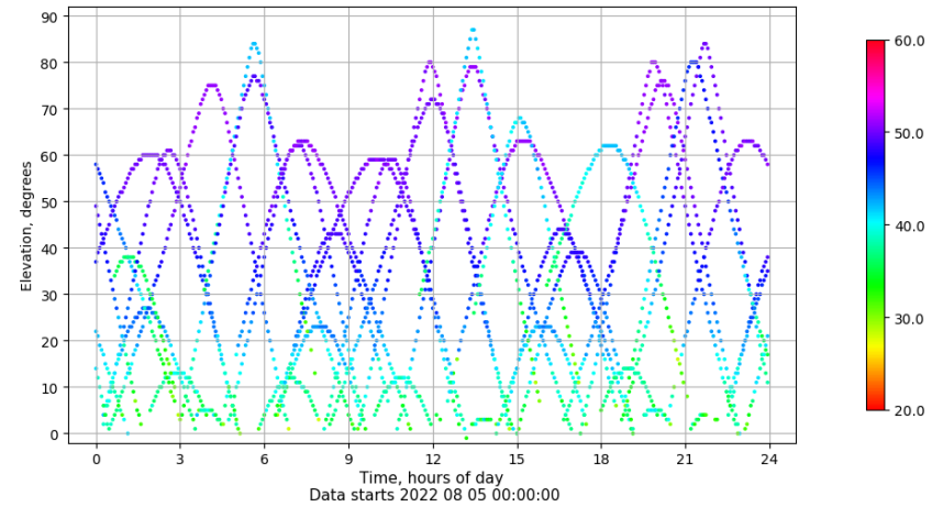
Time-elevation plot for station BCL1. Signal to Noise S1C Data file BCL100ESP_R_2022217.xtr
