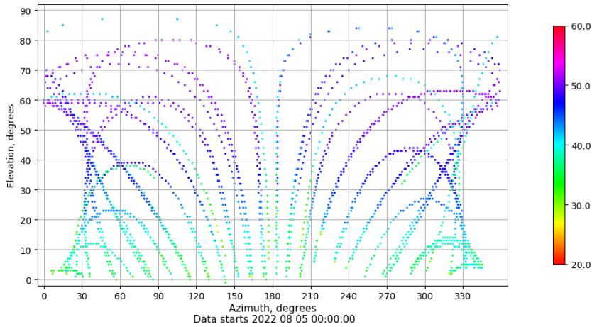
Azimuth-elevation plot for station BCL1. Signal to Noise S1C Data file BCL100ESP_R_2022217.xtr
