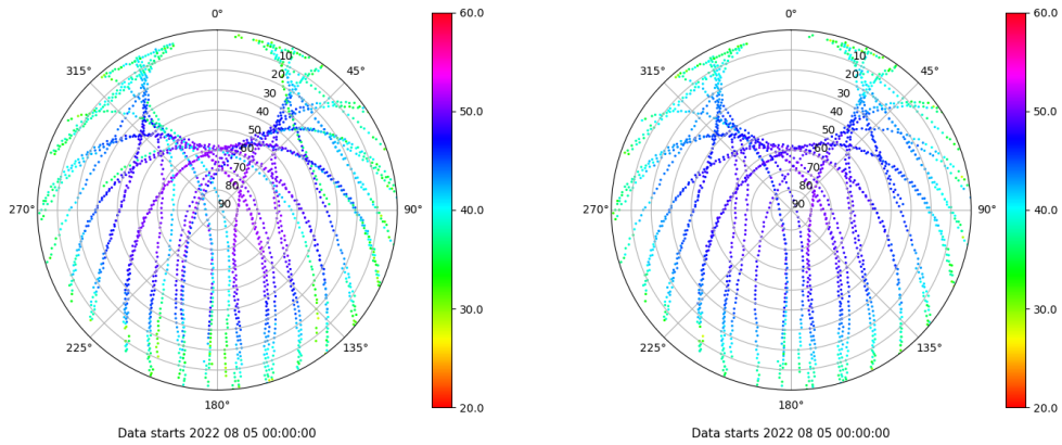
Skyplot for station BCL1. Signal to Noise S1C Data file BCL100ESP_R_2022217.xtr Skyplot for station BCL1. Signal to Noise S2P Data file BCL100ESP_R_2022217.xtr
