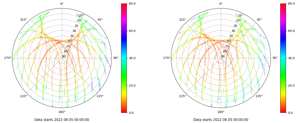
Skyplot for station BCL1. Parameter M1C Data file BCL100ESP_R_2022217.xtr Skyplot for station BCL1. Parameter M2P Data file BCL100ESP_R_2022217.xtr
