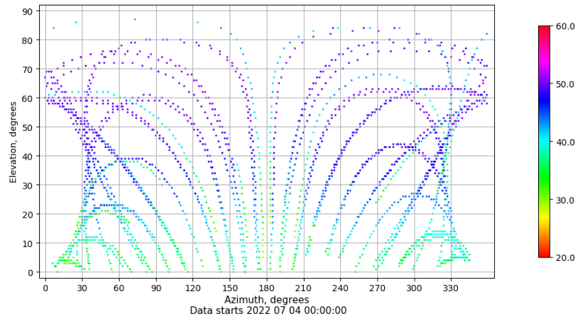
Azimuth-elevation plot for station BCL1. Signal to Noise S1C Data file BCL100ESP_R_2022185.xtr
