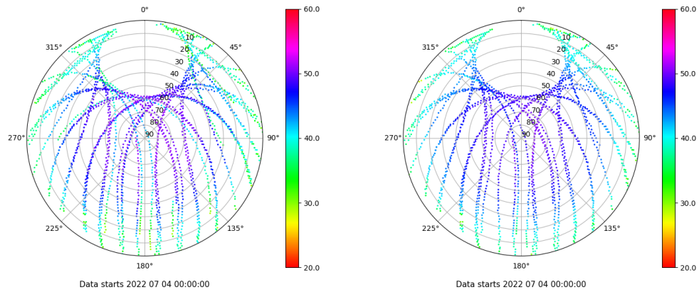
Skyplot for station BCL1. Signal to Noise S1C Data file BCL100ESP_R_2022185.xtr Skyplot for station BCL1. Signal to Noise S2P Data file BCL100ESP_R_2022185.xtr
