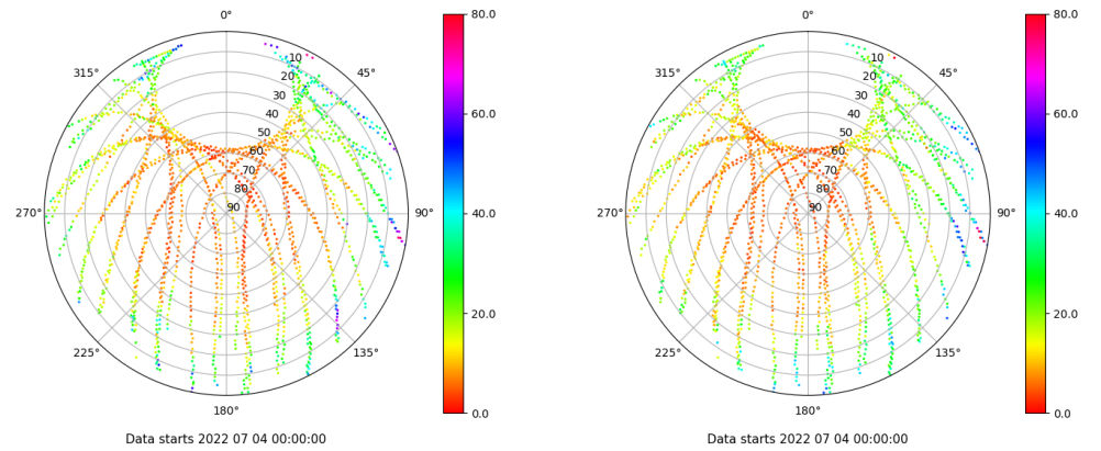
Skyplot for station BCL1. Parameter M1C Data file BCL100ESP_R_2022185.xtr Skyplot for station BCL1. Parameter M2P Data file BCL100ESP_R_2022185.xtr
