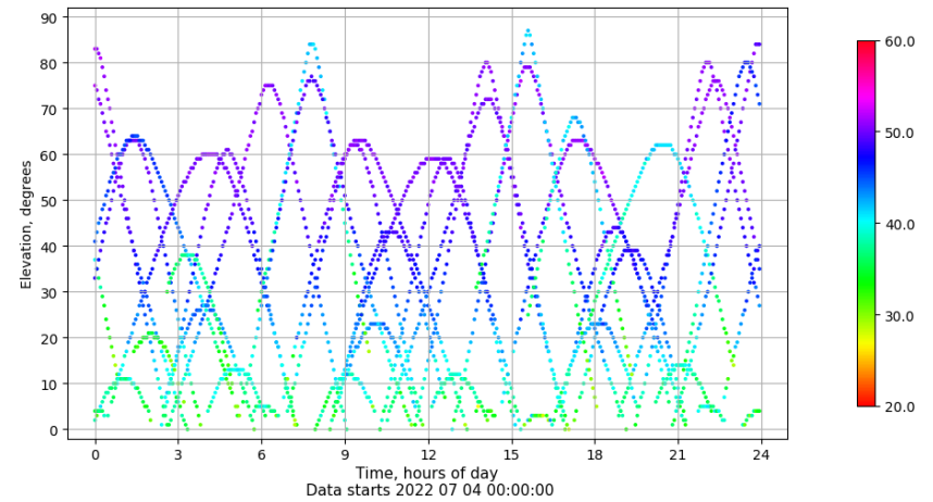
Time-elevation plot for station BCL1. Signal to Noise S1C Data file BCL100ESP_R_2022185.xtr
