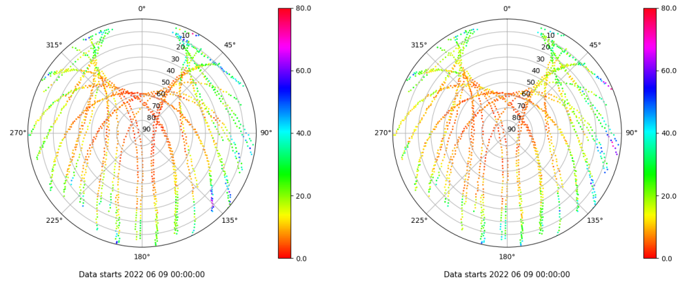
Skyplot for station BCL1. Parameter M1C Data file BCL100ESP_R_2022160.xtr Skyplot for station BCL1. Parameter M2P Data file BCL100ESP_R_2022160.xtr
