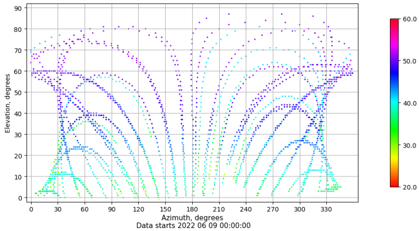
Azimuth-elevation plot for station BCL1. Signal to Noise S1C Data file BCL100ESP_R_2022160.xtr
