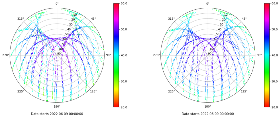
Skyplot for station BCL1. Signal to Noise S1C Data file BCL100ESP_R_2022160.xtr Skyplot for station BCL1. Signal to Noise S2P Data file BCL100ESP_R_2022160.xtr
