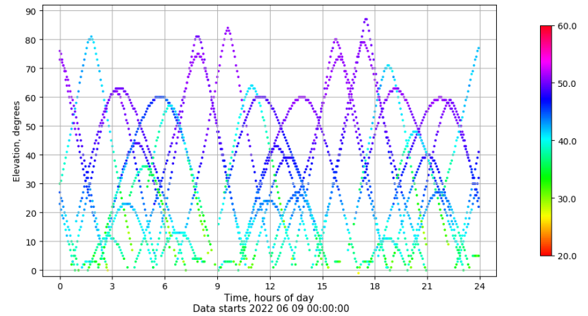
Time-elevation plot for station BCL1. Signal to Noise S1C Data file BCL100ESP_R_2022160.xtr
