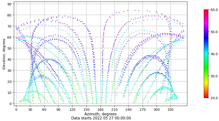
Azimuth-elevation plot for station BCL1. Signal to Noise S1C Data file BCL100ESP_R_2022147.xtr
