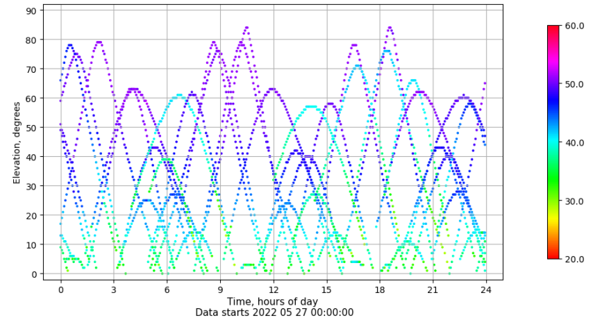
Time-elevation plot for station BCL1. Signal to Noise S1C Data file BCL100ESP_R_2022147.xtr
