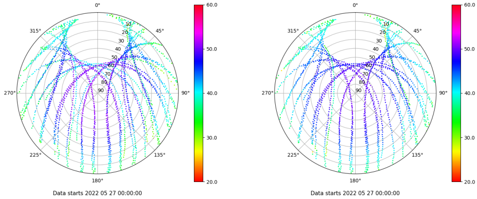
Skyplot for station BCL1. Signal to Noise S1C Data file BCL100ESP_R_2022147.xtr Skyplot for station BCL1. Signal to Noise S2P Data file BCL100ESP_R_2022147.xtr
