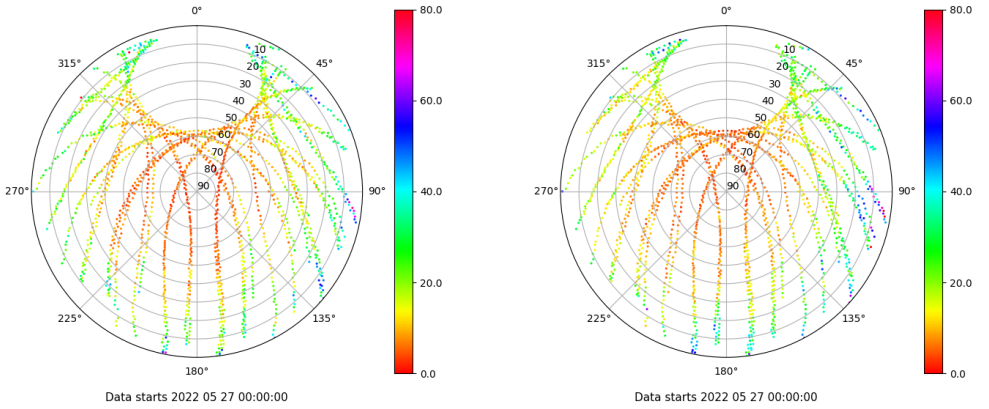
Skyplot for station BCL1. Parameter M1C Data file BCL100ESP_R_2022147.xtr Skyplot for station BCL1. Parameter M2P Data file BCL100ESP_R_2022147.xtr
