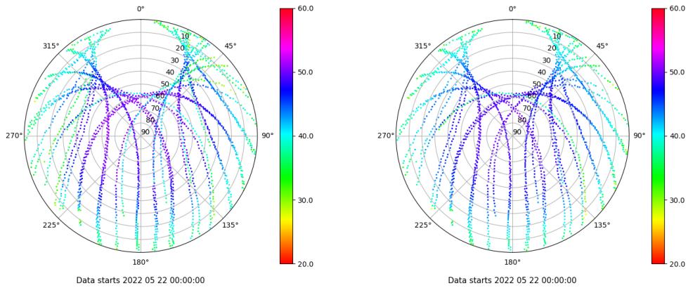
Skyplot for station BCL1. Signal to Noise S1C Data file BCL100ESP_R_2022142.xtr Skyplot for station BCL1. Signal to Noise S2P Data file BCL100ESP_R_2022142.xtr
