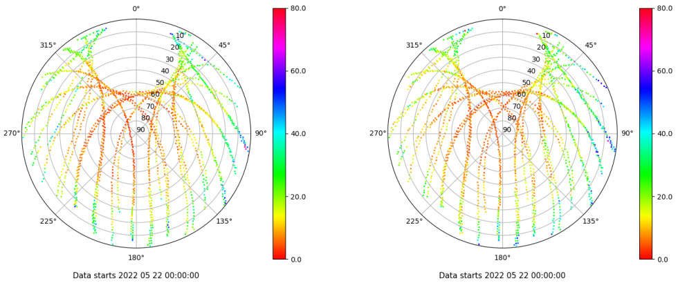
Skyplot for station BCL1. Parameter M1C Data file BCL100ESP_R_2022142.xtr Skyplot for station BCL1. Parameter M2P Data file BCL100ESP_R_2022142.xtr
