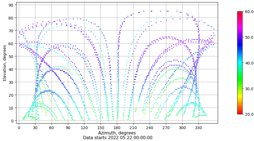
Azimuth-elevation plot for station BCL1. Signal to Noise S1C Data file BCL100ESP_R_2022142.xtr
