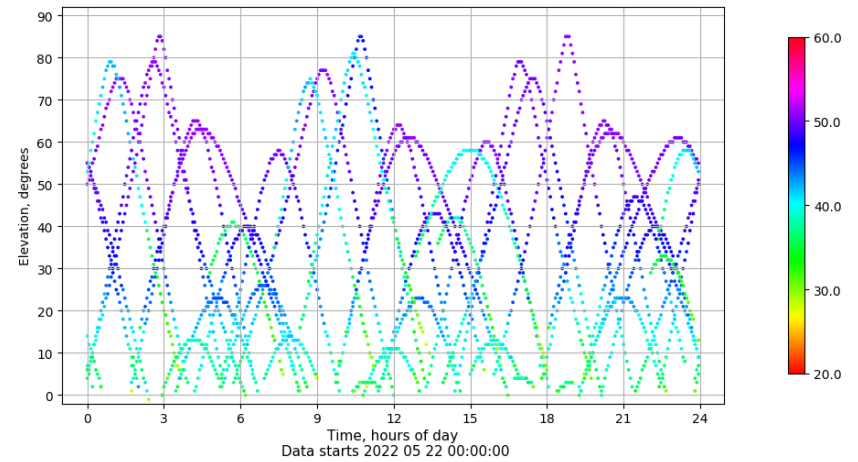
Time-elevation plot for station BCL1. Signal to Noise S1C Data file BCL100ESP_R_2022142.xtr
