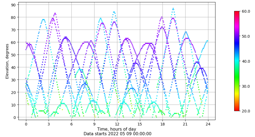
Time-elevation plot for station BCL1. Signal to Noise S1C Data file BCL100ESP_R_2022129.xtr
