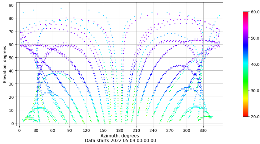
Azimuth-elevation plot for station BCL1. Signal to Noise S1C Data file BCL100ESP_R_2022129.xtr
