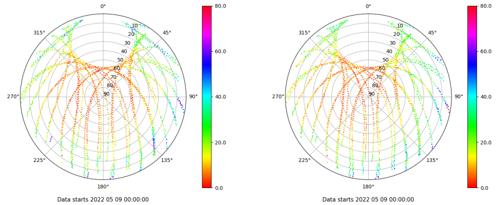
Skyplot for station BCL1. Parameter M1C Data file BCL100ESP_R_2022129.xtr Skyplot for station BCL1. Parameter M2P Data file BCL100ESP_R_2022129.xtr
