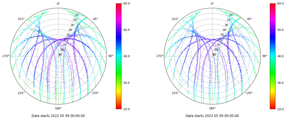
Skyplot for station BCL1. Signal to Noise S1C Data file BCL100ESP_R_2022129.xtr Skyplot for station BCL1. Signal to Noise S2P Data file BCL100ESP_R_2022129.xtr
