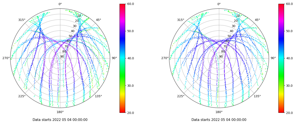
Skyplot for station BCL1. Signal to Noise S1C Data file BCL100ESP_R_2022124.xtr Skyplot for station BCL1. Signal to Noise S2P Data file BCL100ESP_R_2022124.xtr
