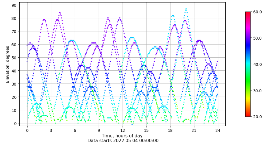
Time-elevation plot for station BCL1. Signal to Noise S1C Data file BCL100ESP_R_2022124.xtr
