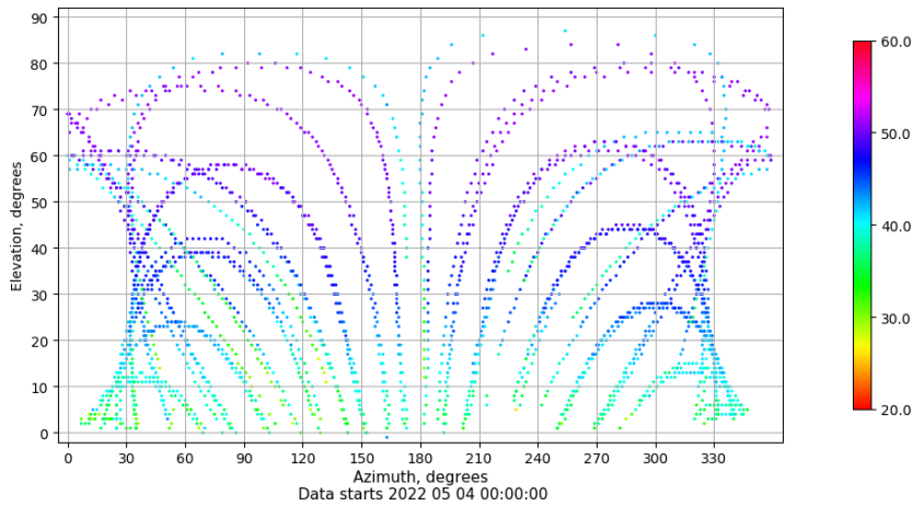
Azimuth-elevation plot for station BCL1. Signal to Noise S1C Data file BCL100ESP_R_2022124.xtr
