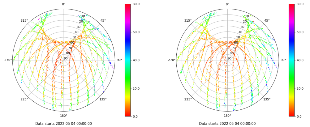
Skyplot for station BCL1. Parameter M1C Data file BCL100ESP_R_2022124.xtr Skyplot for station BCL1. Parameter M2P Data file BCL100ESP_R_2022124.xtr
