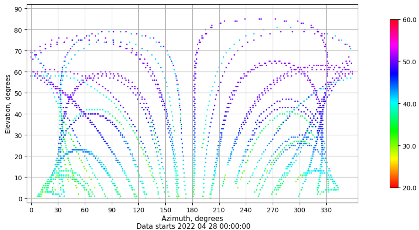
Azimuth-elevation plot for station BCL1. Signal to Noise S1C Data file BCL100ESP_R_2022118.xtr
