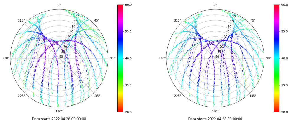
Skyplot for station BCL1. Signal to Noise S1C Data file BCL100ESP_R_2022118.xtr Skyplot for station BCL1. Signal to Noise S2P Data file BCL100ESP_R_2022118.xtr
