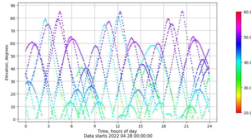
Time-elevation plot for station BCL1. Signal to Noise S1C Data file BCL100ESP_R_2022118.xtr
