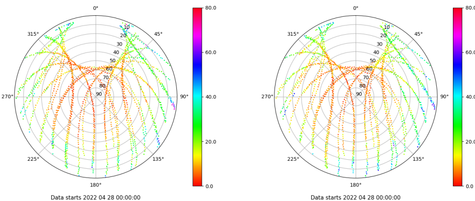
Skyplot for station BCL1. Parameter M1C Data file BCL100ESP_R_2022118.xtr Skyplot for station BCL1. Parameter M2P Data file BCL100ESP_R_2022118.xtr
